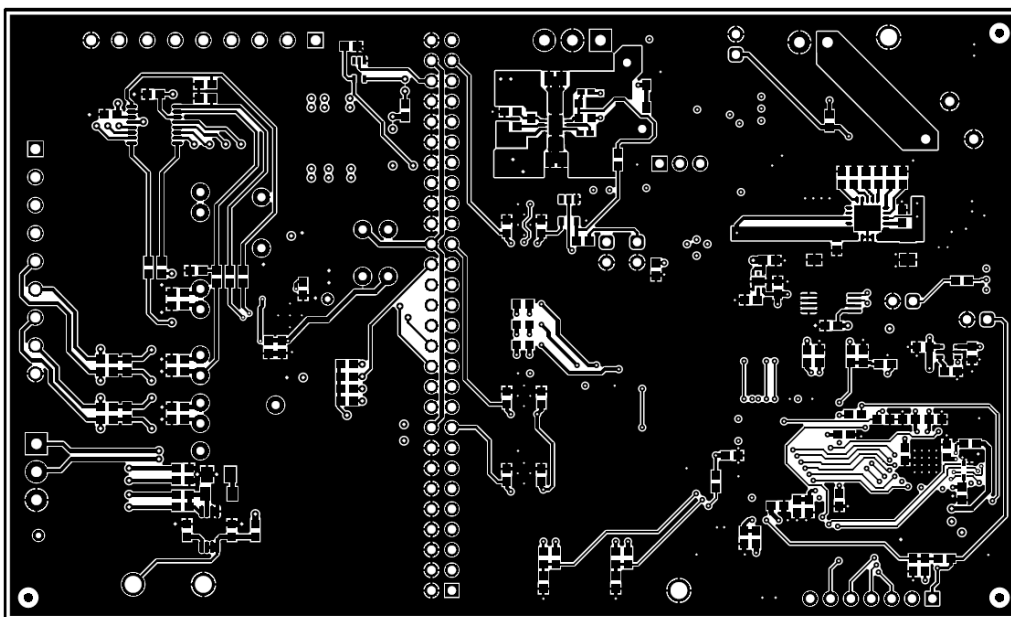
Figure 16. Bottom Layer (Positive)
