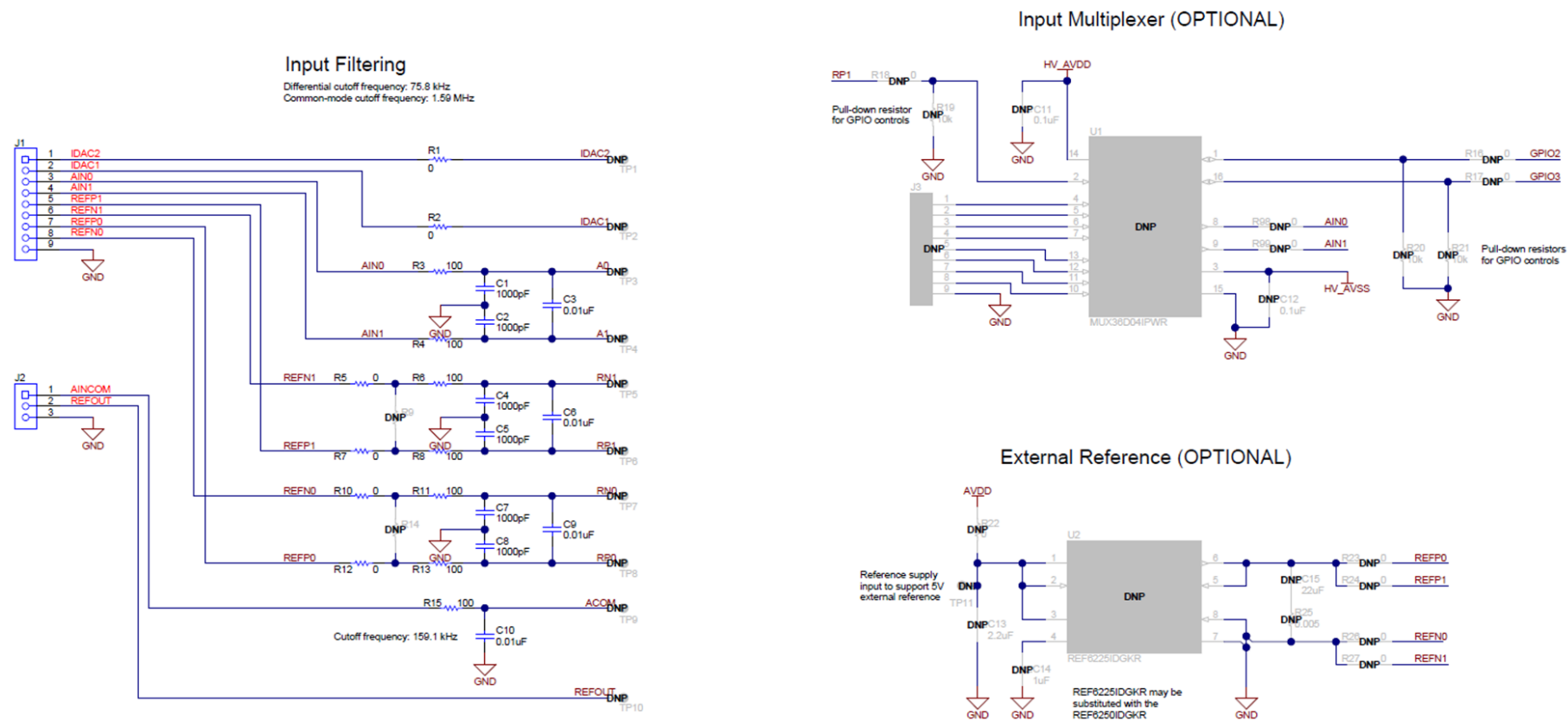
Figure 19. ADS125H02EVM Analog Inputs Header Schematic
