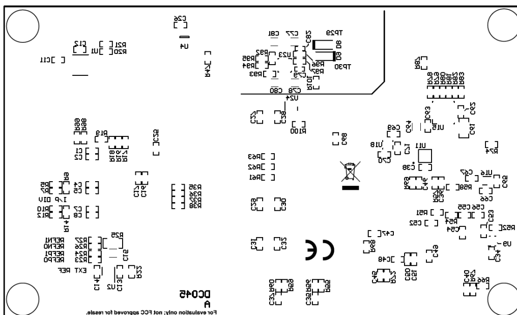
Figure 17. Bottom Silkscreen
