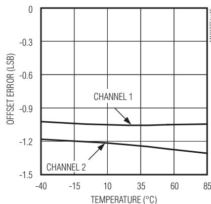
MAX1379 OFFSET ERROR vs. TEMPERATURE
