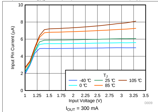
Figure 19. I_Q ( V_{IN} ) Over Temperature
