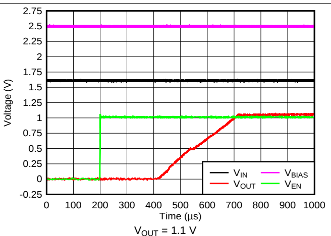
Figure 22. Startup With Separated V_{EN}
