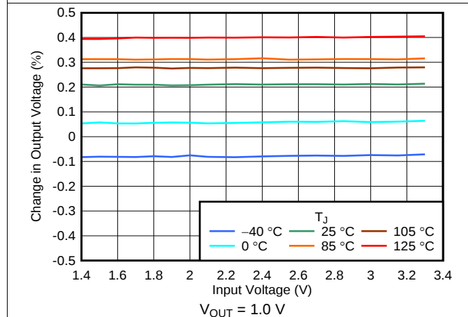
Figure 3. Output Accuracy Over Temperature, DSE Package
