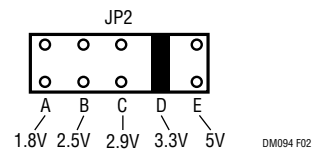
Figure 2. Output Voltage Selection (JP2) (3.3V Position Shown)
