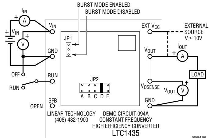
Figure 3. Proper Measurement Setup
