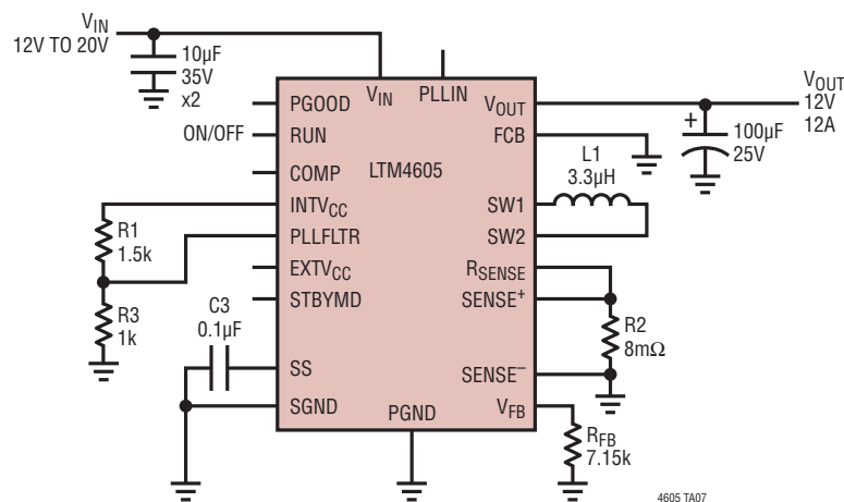
Buck Mode Operation with 12V to 20V Input
