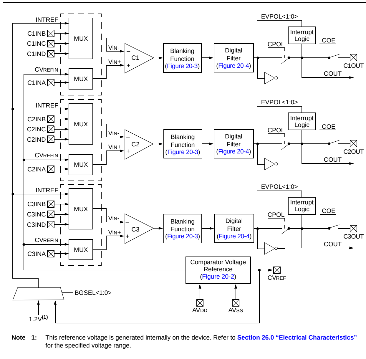
FIGURE 20-1: COMPARATOR I/O OPERATING MODES
