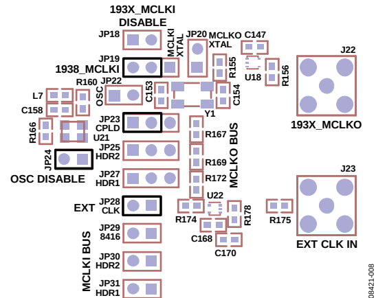
Figure 8. External Clock In as Master; the AD1938 and CPLD as Slaves
