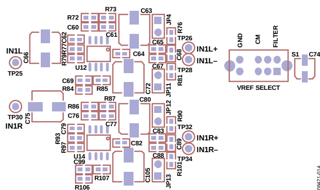
Figure 14. VREF Selection and DC Coupling Jumpers
