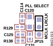
Figure 13. LRCLK Loop Filter Selected
