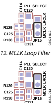
Figure 13. LRCLK Loop Filter Selected
