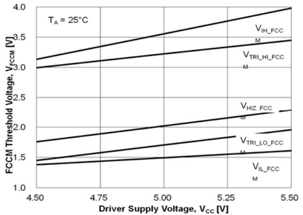
Figure 19. FCCM Threshold vs. Driver Supply Voltage
