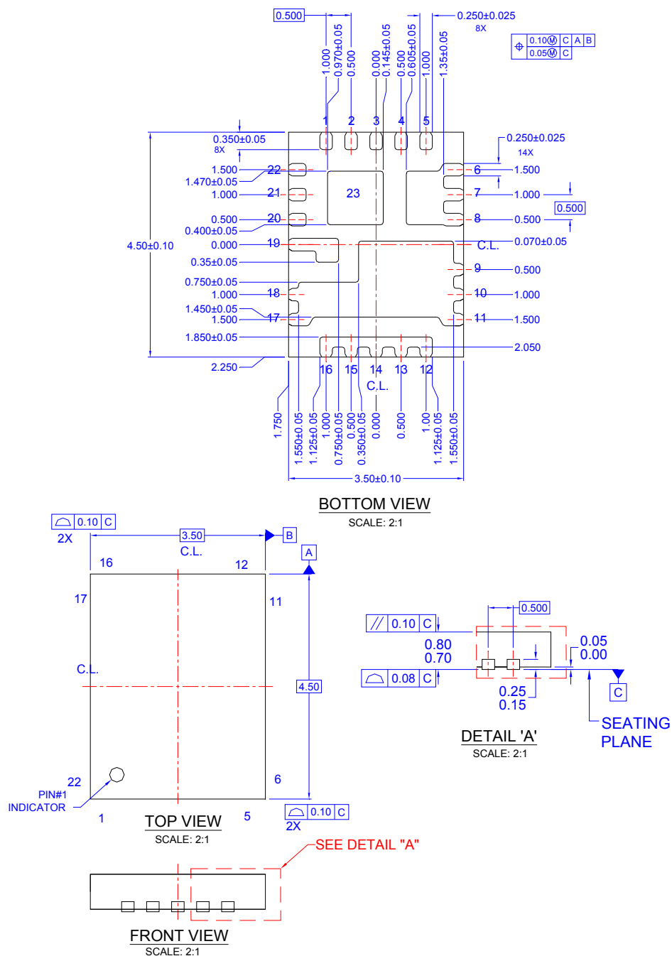
Figure 34. 22-Lead, Clip Bond PQFN SPS, 3.5 mm x 4.5 mm Package Physical Dimension
