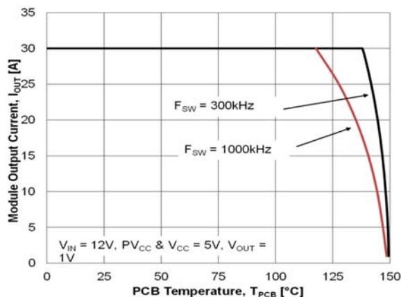
Figure 4. Safe Operating Area with 12 V_{IN}
