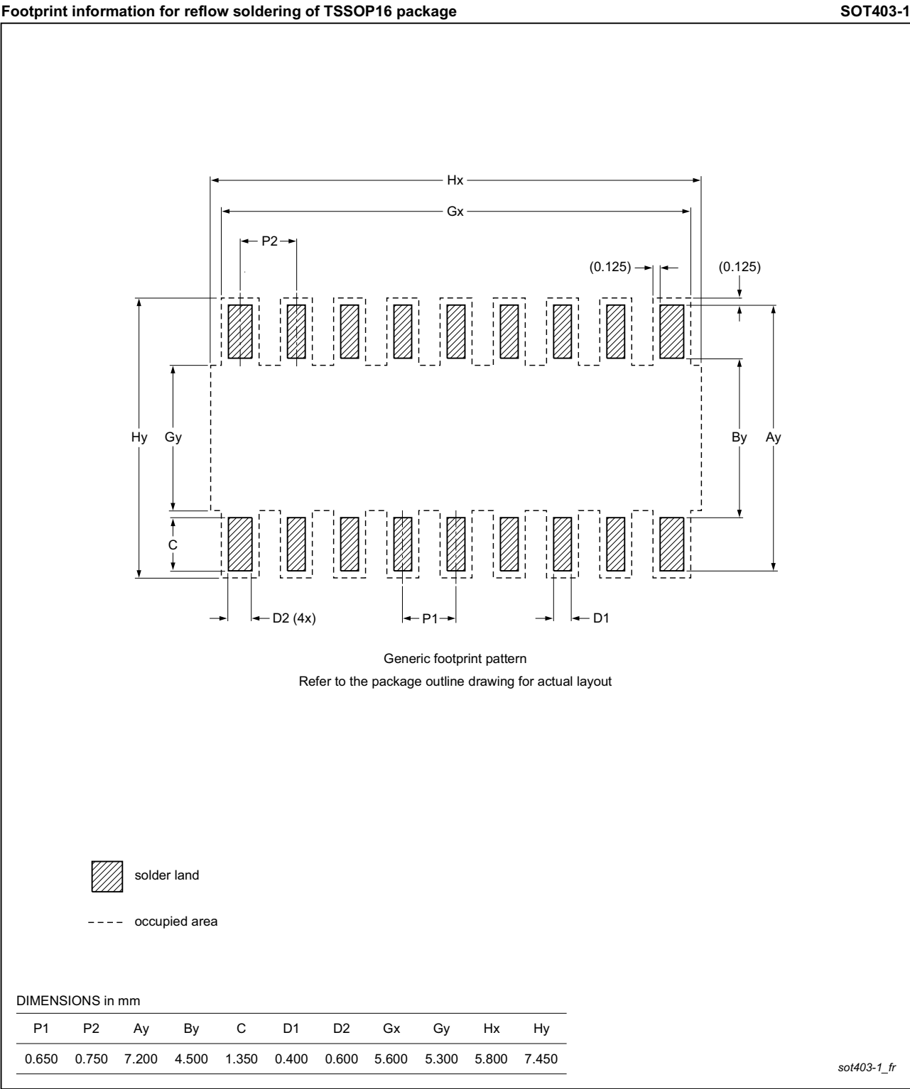
Fig 24. PCB footprint for SOT403-1 (TSSOP16); reflow soldering
