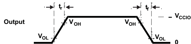
Figure 7-2. CMOS-Level Outputs
