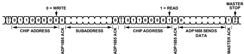
Figure 32. I²C Single Register Read Sequence
