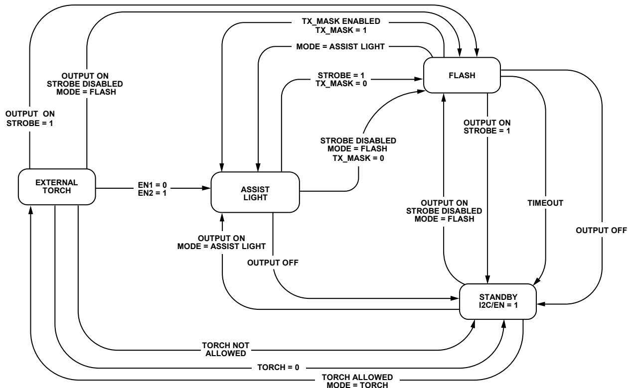
Figure 34. I2C Interface Mode: State Transitions
