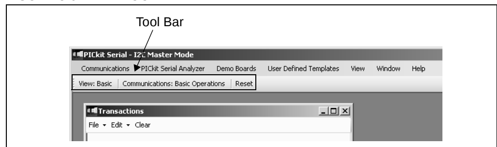
FIGURE 3-9: TOOL BAR
