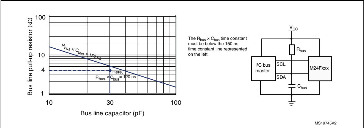
Figure 12. Maximum R_{bus} value versus bus parasitic capacitance ( C_{bus} ) for an I 2 C bus at maximum frequency f_c = 1\text{ MHz}
