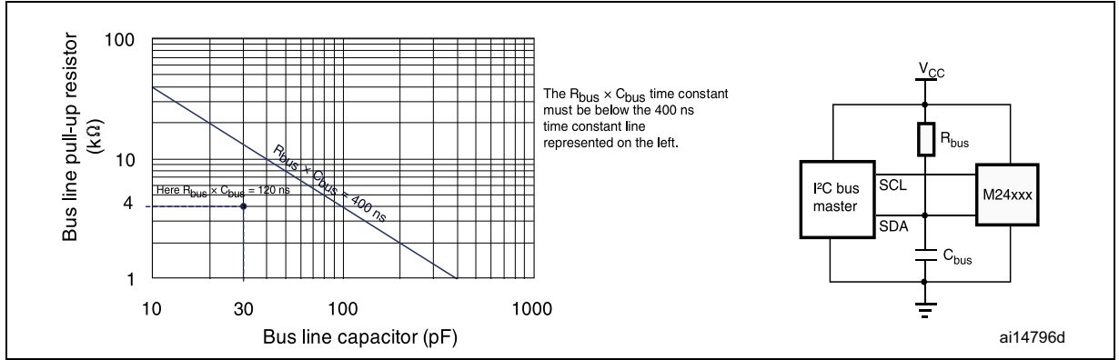
Figure 13. Maximum R_{bus} value versus bus parasitic capacitance ( C_{bus} ) for an I 2 C bus at maximum frequency f_c = 400\text{ kHz}
