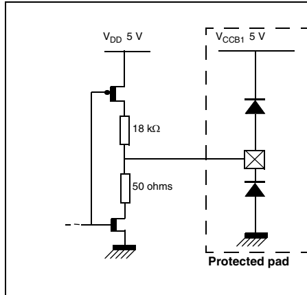
Figure 10. C gate logical output (pin 52)
