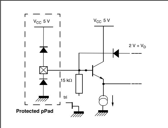
Figure 8. Fast blanking inputs (pins 50, 51)
