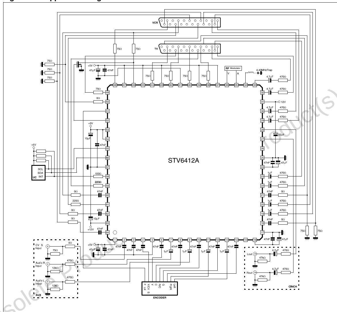
Figure 22. Application diagram
