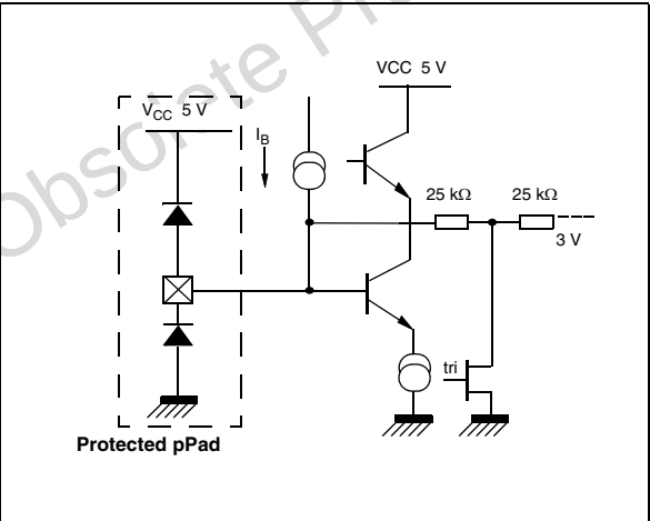
Figure 9. Average clamped video inputs (pin 8)
