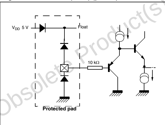
Figure 19. 2 C bus (ADD) (pin 54)
