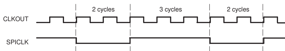
Figure 12-5. SPI: SPICLK-CLKOUT Characteristic When (BRR + 1) is Odd, BRR > 3, and CLOCK POLARITY = 1
