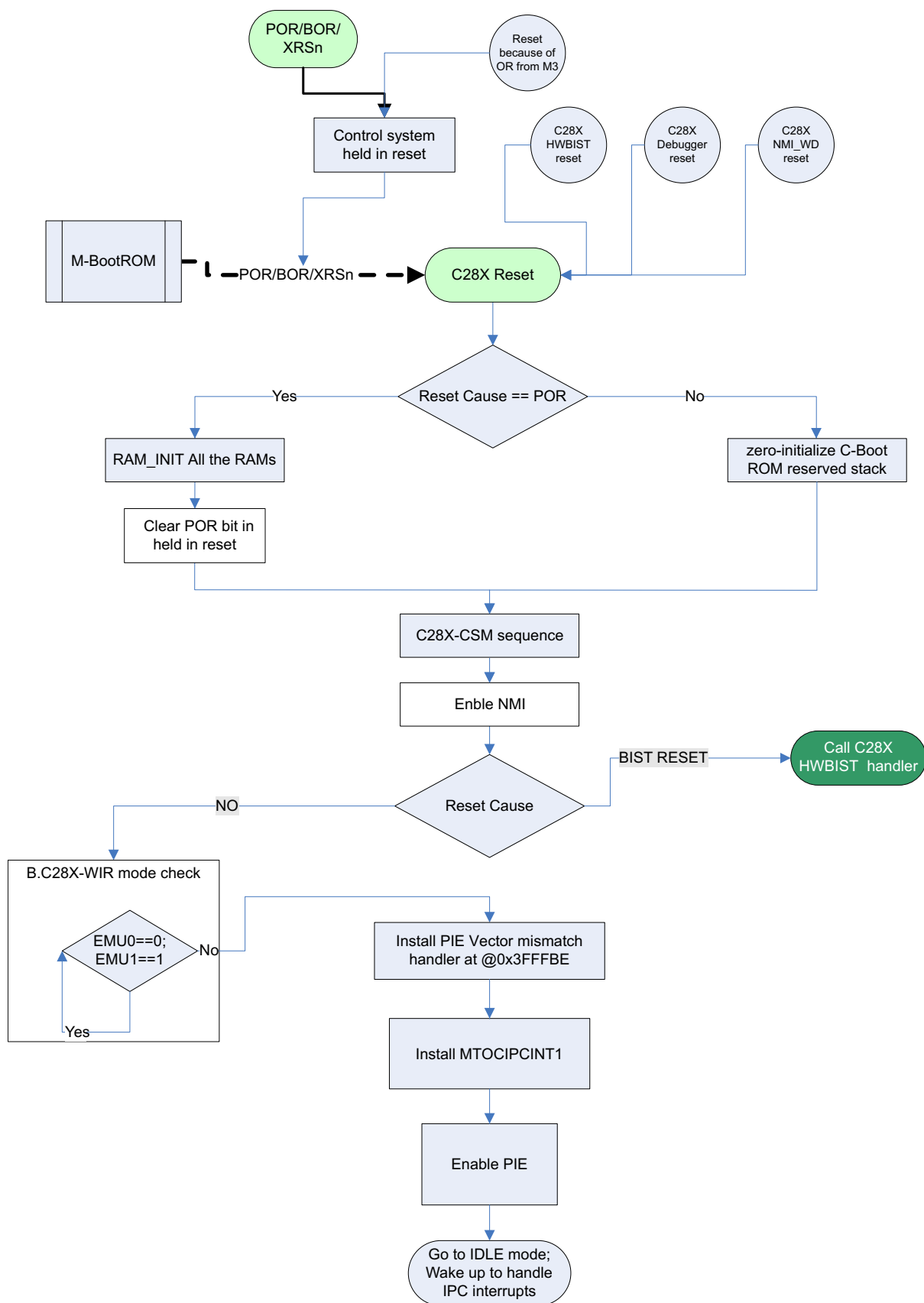
Figure 6-12. C-Boot ROM Flow Chart
