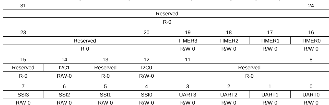
Figure 1-109. Sleep Mode Clock Gating Control Register 1 (SCGC1)
