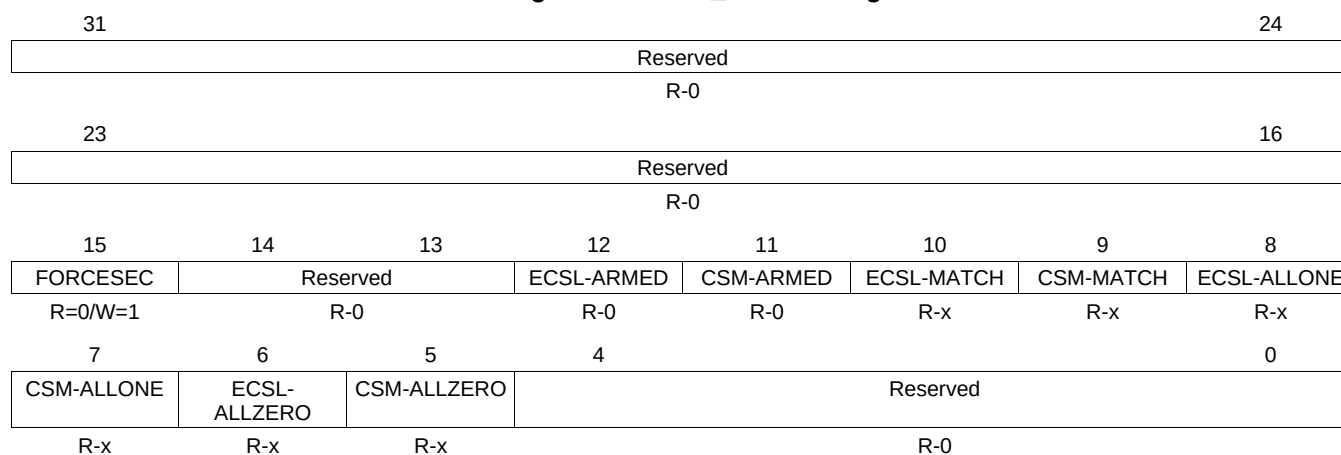
Figure 1-138. Z1_CSMCR Register
