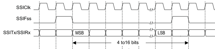
Figure 20-3. TI Synchronous Serial Frame Format (Continuous Transfer)
