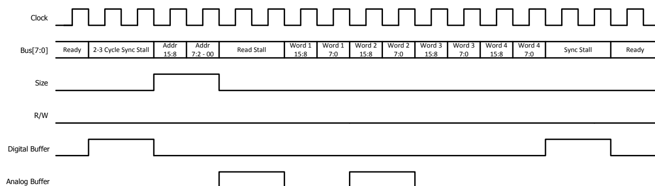
Figure 10-7. 64-bit Read
