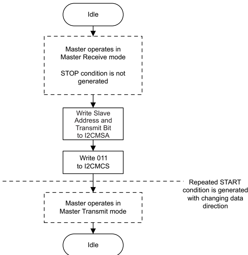
Figure 22-12. Master TRANSMIT with Repeated START after RECEIVE with Repeated START
