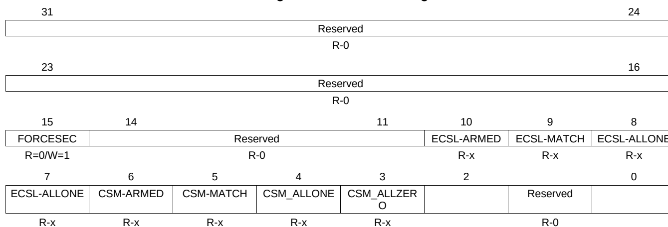
Figure 1-151. CSMCR Register
