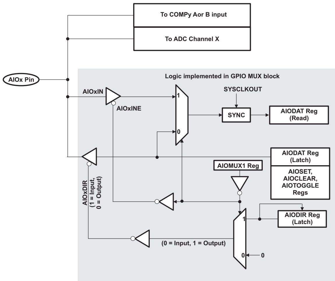
Figure 4-38. Analog/GPIO Multiplexing
