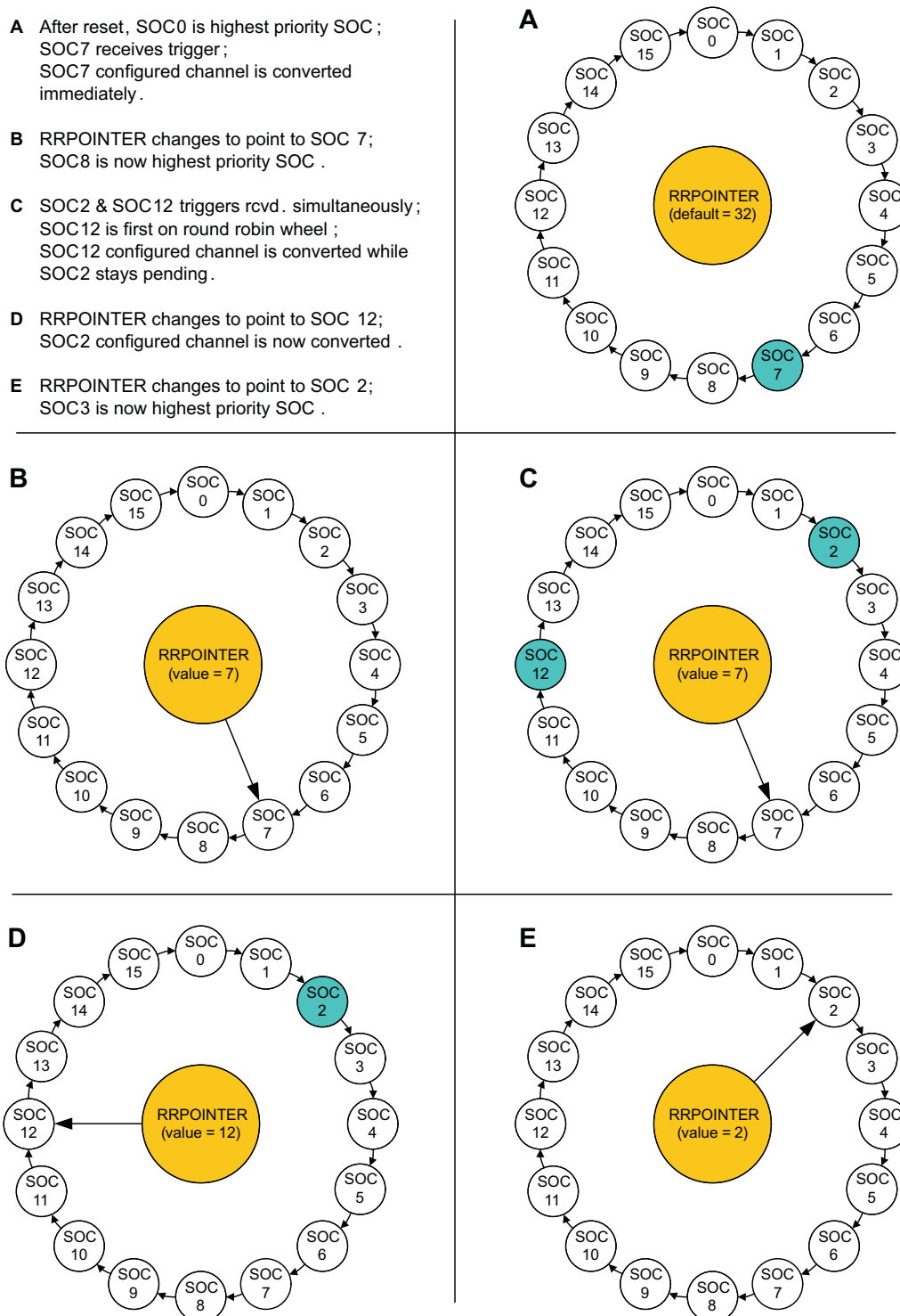
Figure 10-14. Round Robin Priority Example
