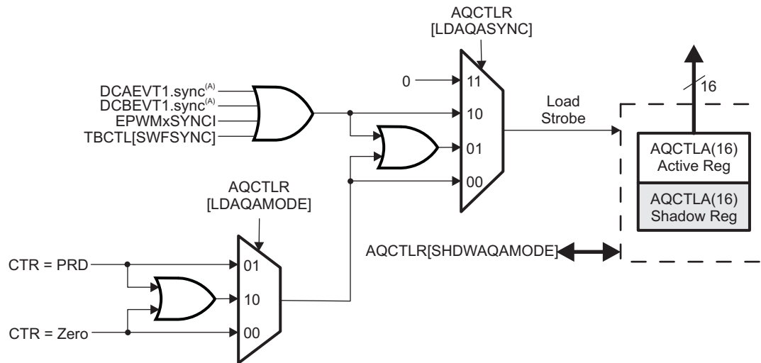
Figure 7-21. AQCTLR[SHDWAQAMODE]
