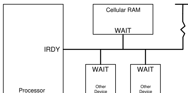
Figure 17-6. iRDY Signal Connection
