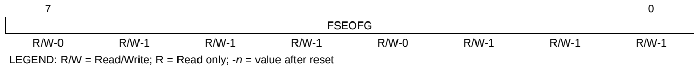
Figure 18-25. USB Full-Speed Last Transaction to End of Frame Timing Register (USBFSEOF)
