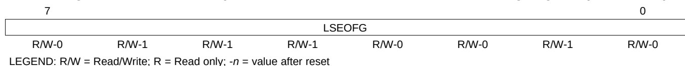
Figure 18-26. USB Low-Speed Last Transaction to End of Frame Timing Register (USBLSEOF)
