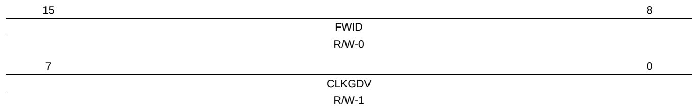
Figure 15-73. Sample Rate Generator 1 Register (SRGR1)
