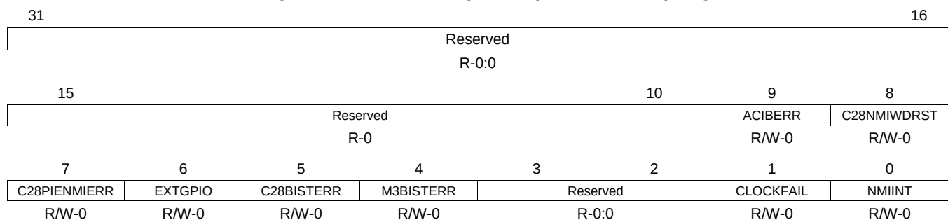
Figure 1-60. M3NMI Flag Clear (NMIFLGCLR) Register
