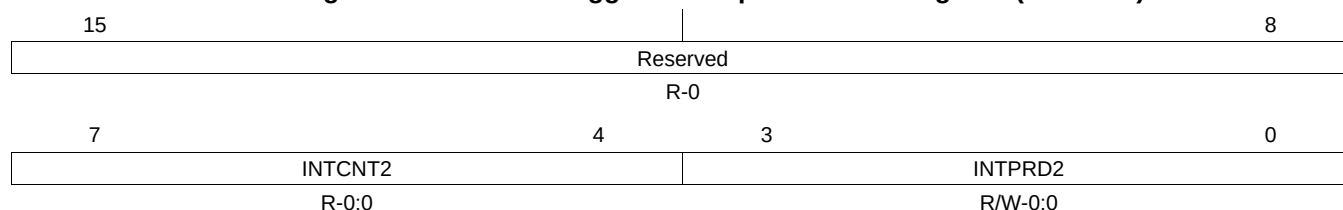
Figure 7-134. Event-Trigger Interrupt Pre-Scale Register (ETINTPS)
