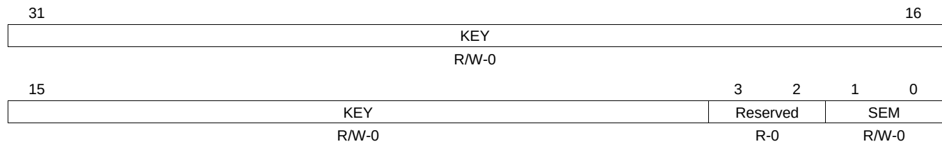
Figure 5-90. SECZONEREQUEST(SEM) Register
