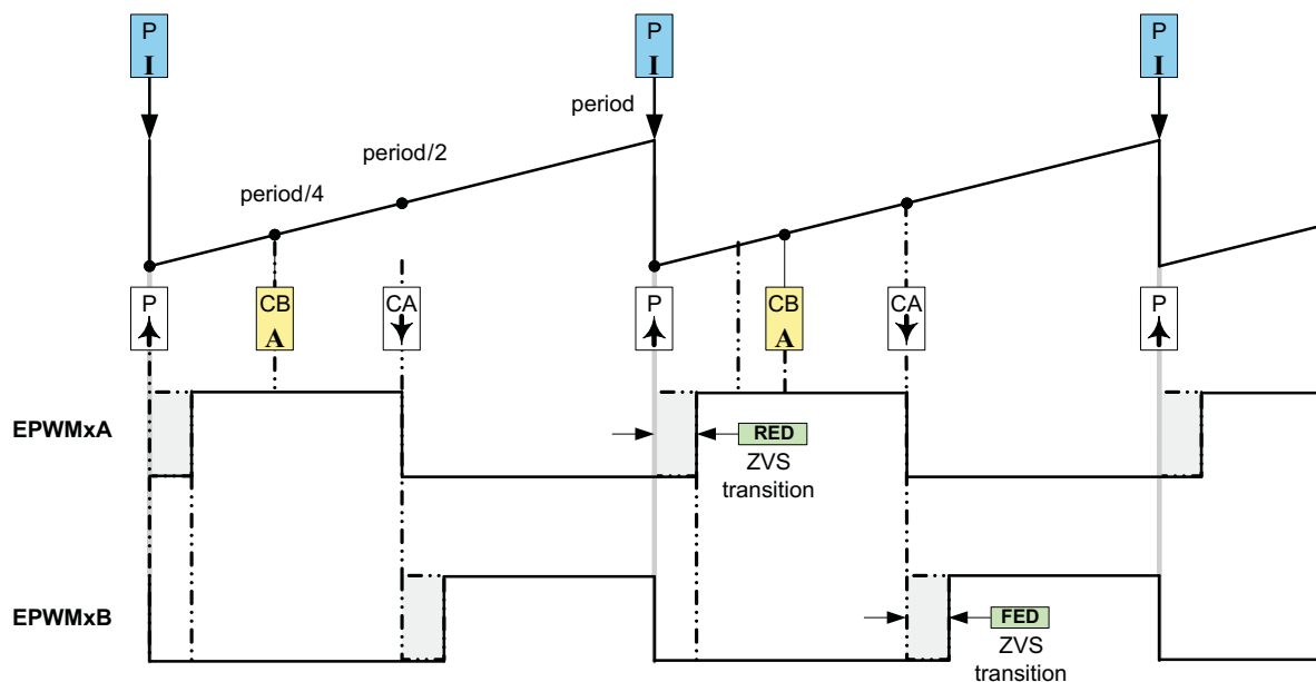
Figure 7-74. H-Bridge LLC Resonant Converter PWM Waveforms
