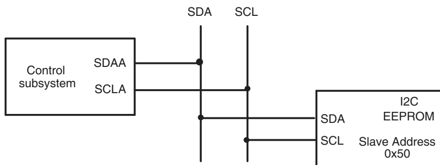
Figure 6-24. EEPROM Device at Address 0x50
