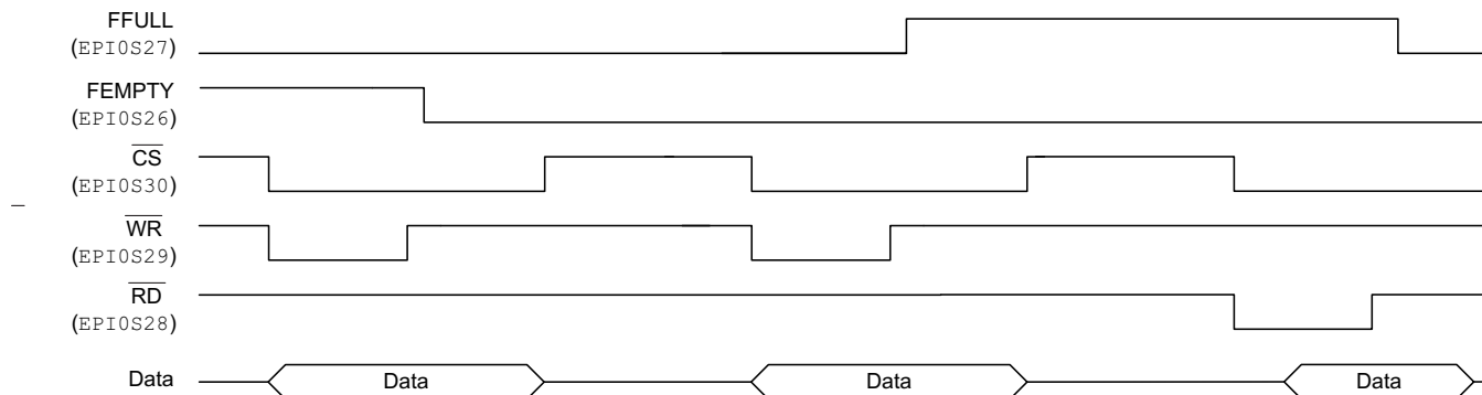
Figure 17-14. Two-Entry FIFO
