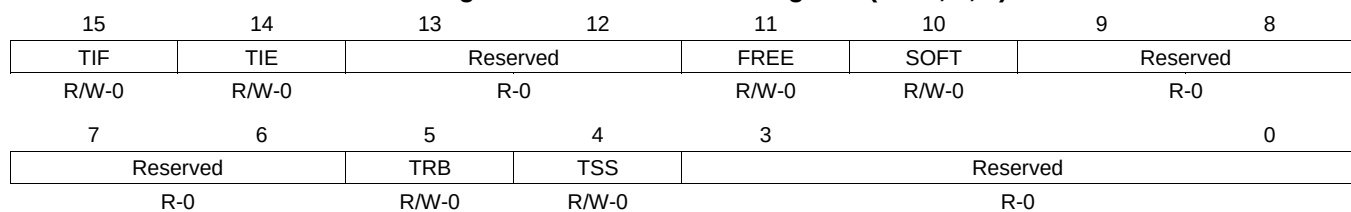
Figure 1-20. TIMERxTCR Register (x = 0, 1, 2)
