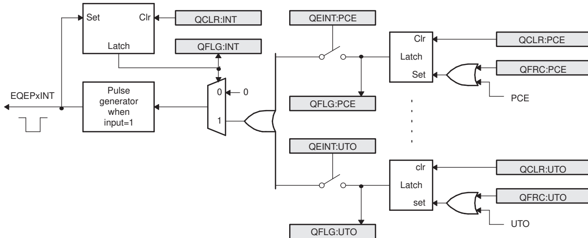
Figure 9-20. EQEP Interrupt Generation
