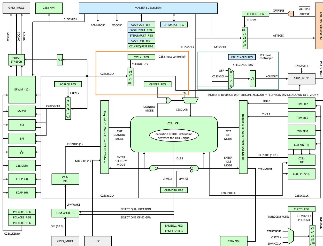
Figure 1-12. Control Subsystem Clocks and Low Power Mode Configuration
