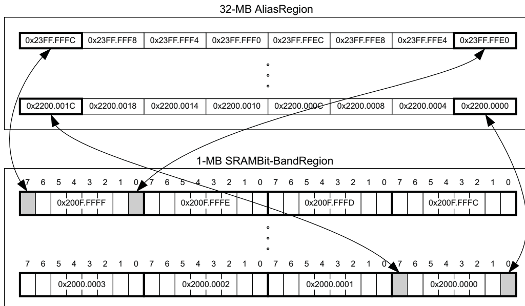
Figure 24-12. Bit-Band Mapping
