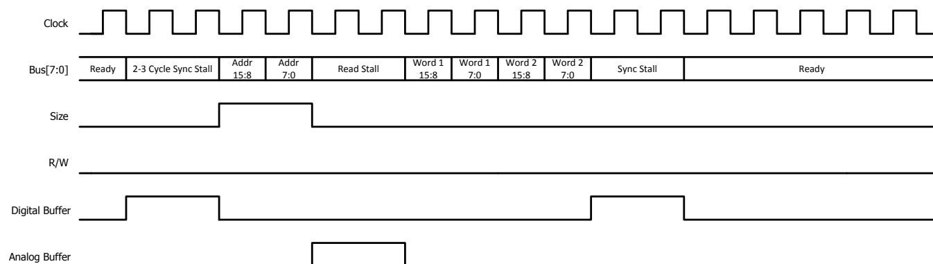
Figure 10-6. 32-bit Read
