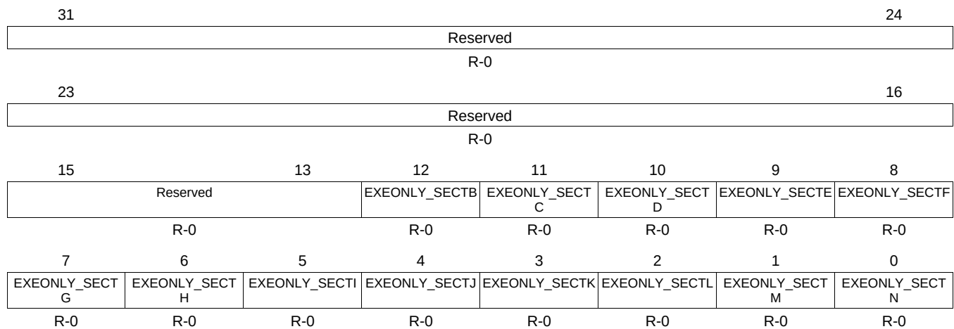
Figure 1-144. Z1_EXEONLYR Register
