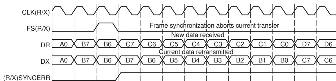
Figure 15-43. Unexpected Frame-Synchronization Pulse With (R/X)FIG = 0
