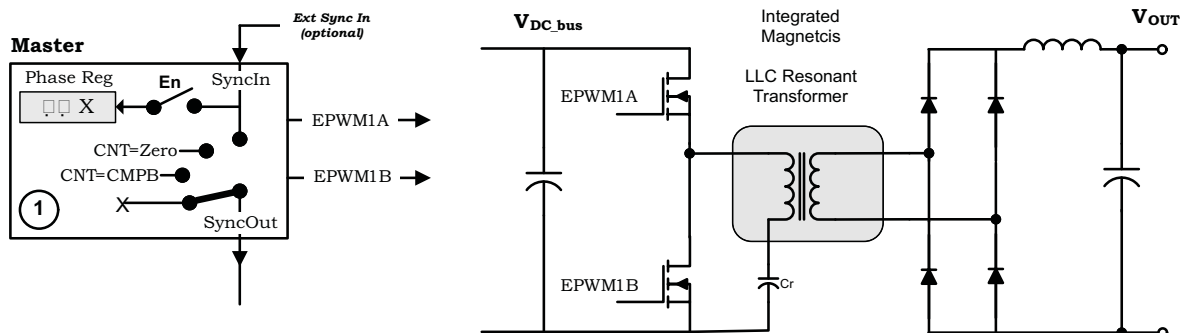
Figure 7-73. Control of Two Resonant Converter Stages
