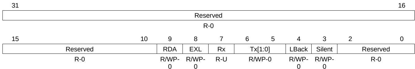
Figure 23-24. Test Register (CAN TEST) [offset = 0x14]
