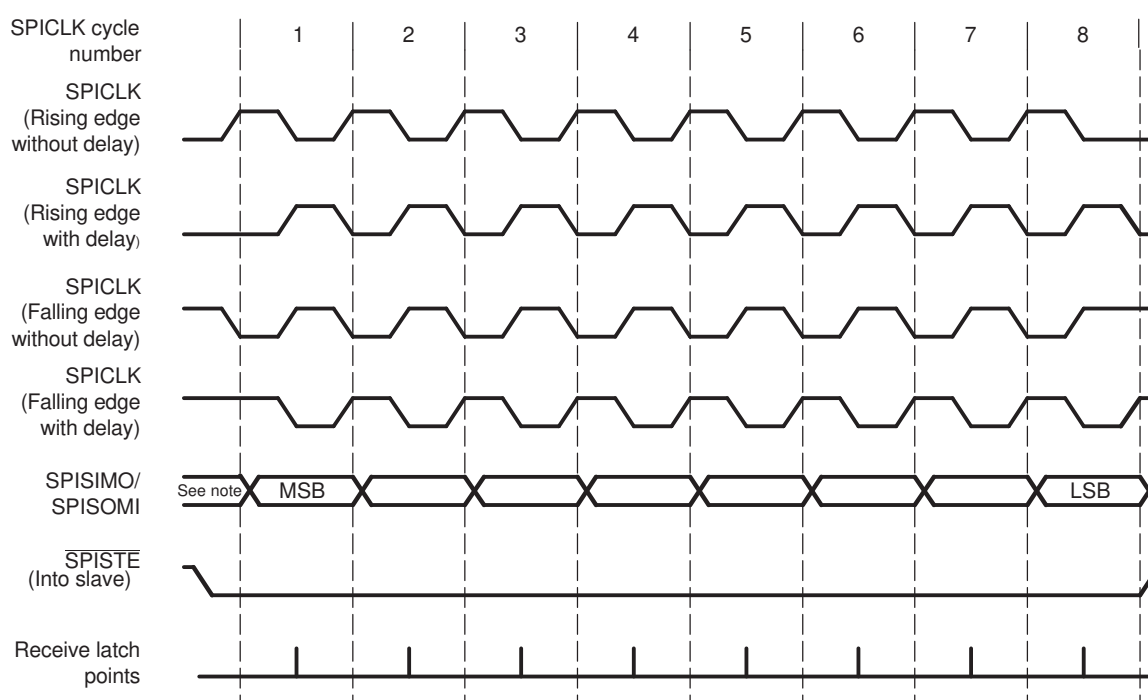
Figure 12-4. SPICLK Signal Options
