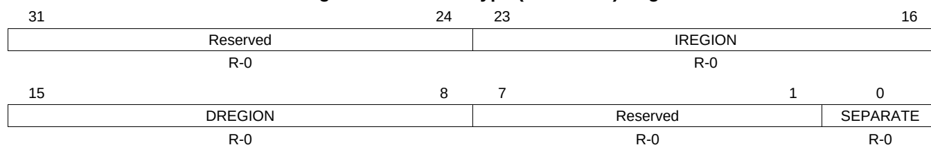
Figure 25-47. MPU Type (MPUTYPE) Register
