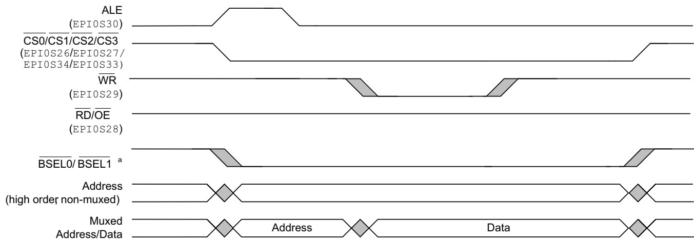
Figure 17-11. Host-Bus Write Cycle with Multiplexed Address and Data and ALE with Dual or Quad \overline{\text{CS}}
