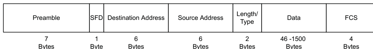
Figure 19-3. Ethernet Frame
