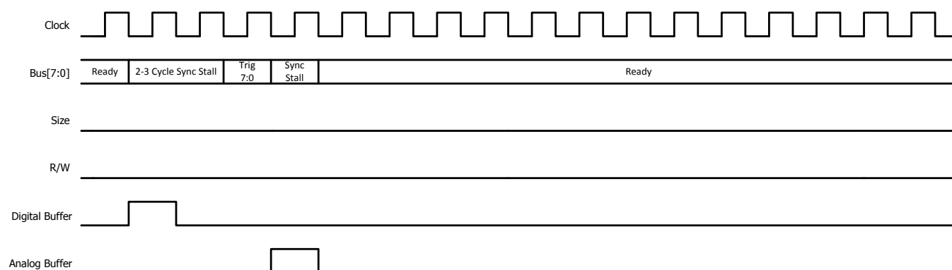
Figure 10-8. ADC Trigger
