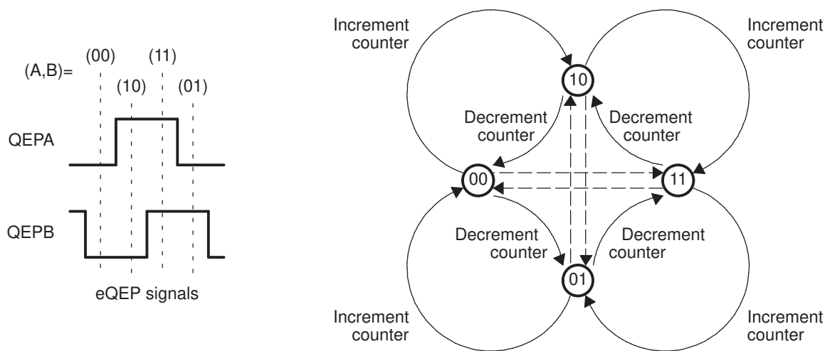
Figure 9-6. Quadrature Decoder State Machine
