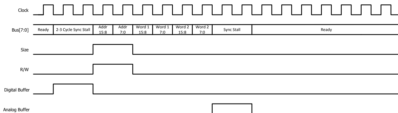
Figure 10-4. 32-bit Write
