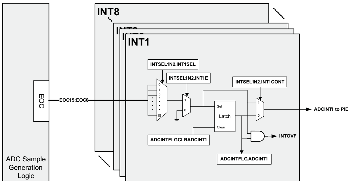
Figure 10-16. Interrupt Structure
