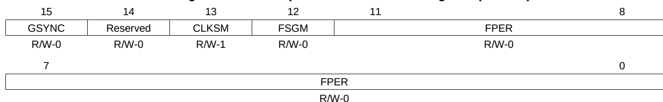
Figure 15-74. Sample Rate Generator 2 Register (SRGR2)
