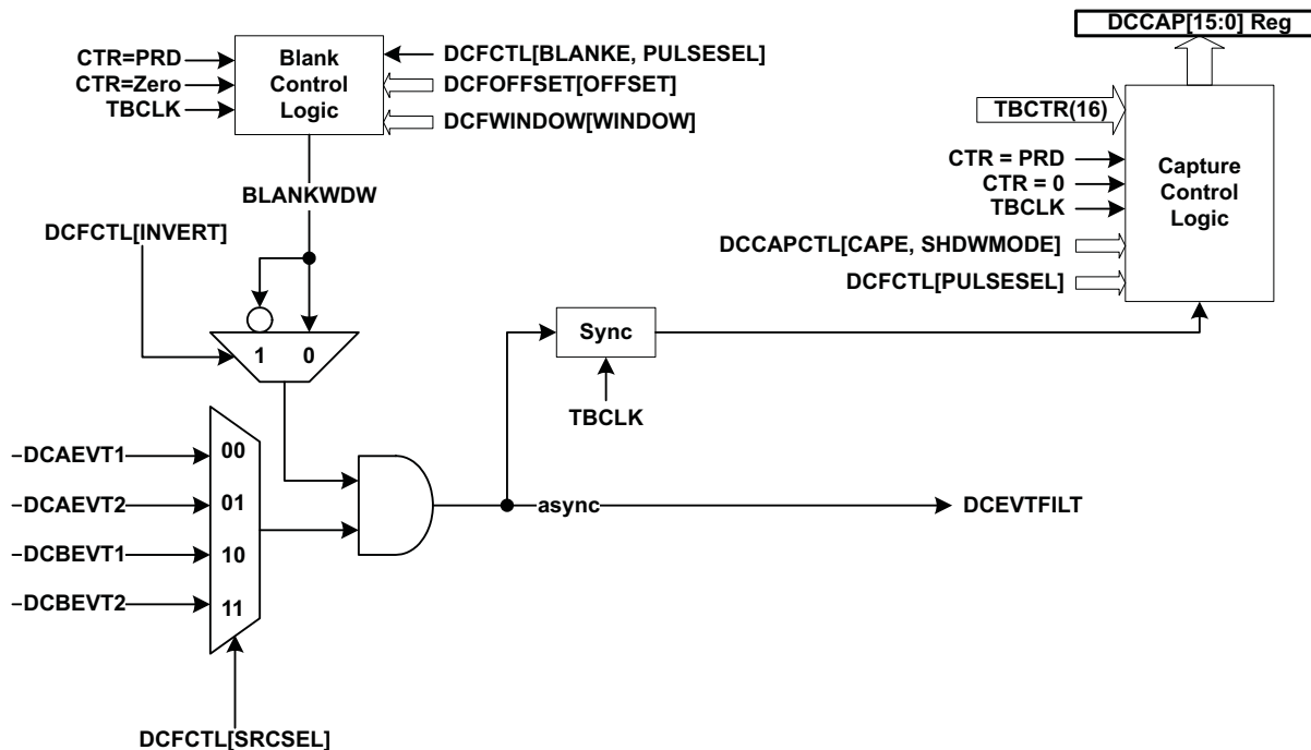
Figure 7-53. Event Filtering
