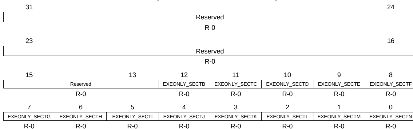
Figure 1-145. Z2_EXEONLYR Register
