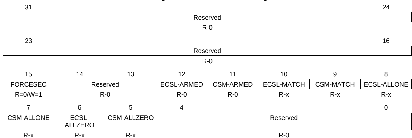
Figure 1-139. Z2_CSMCR Register
