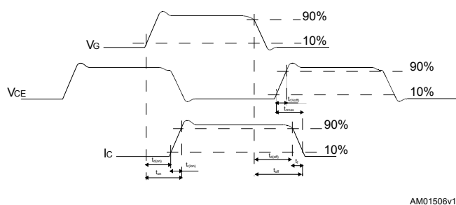
Figure 29. Switching waveform
