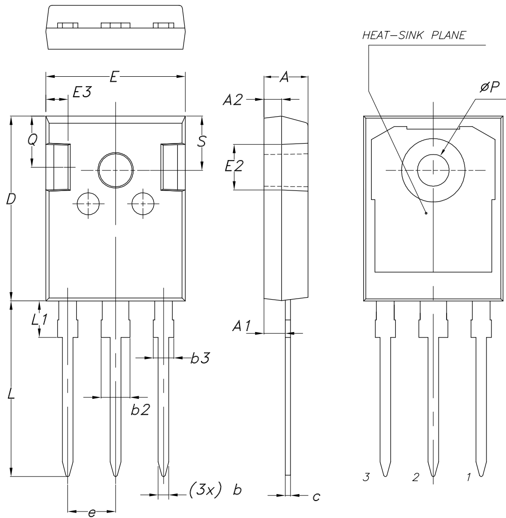
Figure 31. TO-247 long leads package outline
