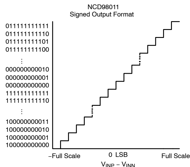
Figure 17. NCD98011 Signed Output Definition
