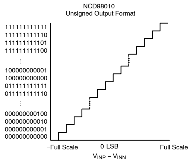
Figure 16. NCD98010 Unsigned Output Definition
