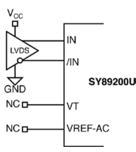
Figure 11. LVDS Interface
