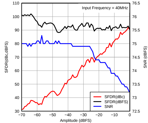
Figure 37. Performance vs Input Amplitude
