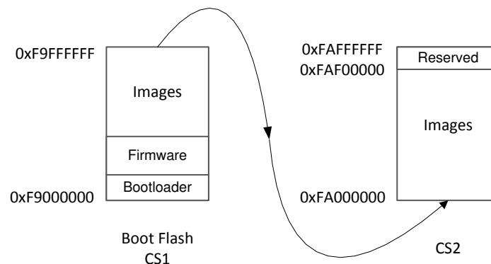
Figure 24. Two 16-Mbit Flash Memory Components
