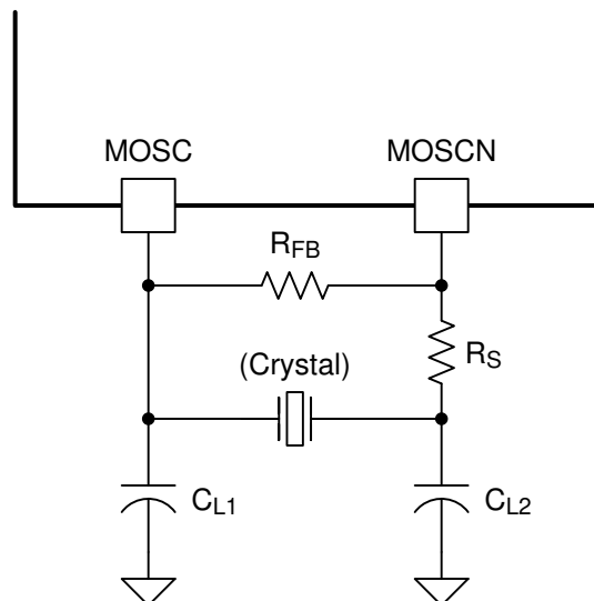
Figure 40. Crystal Oscillator Configuration
