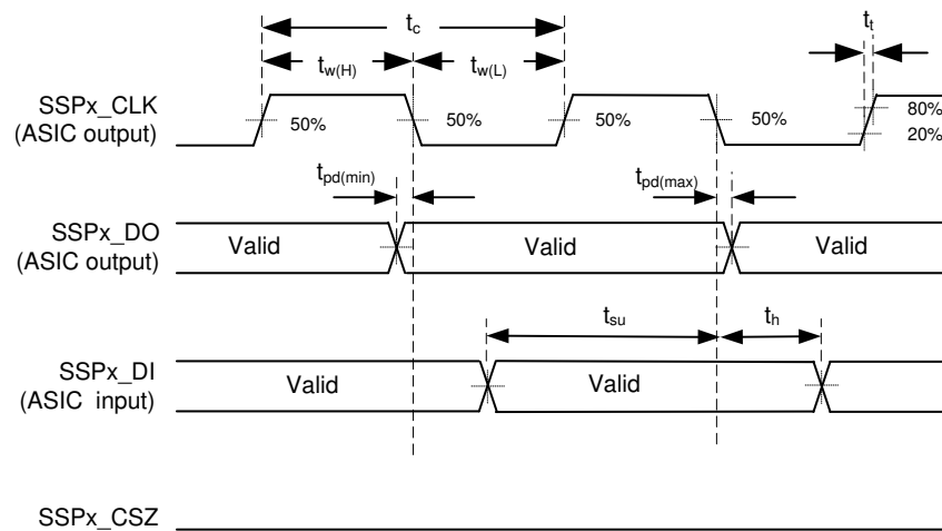
Figure 10. Synchronous Serial Port Interface – Master (Modes 0/3)
