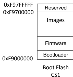
Figure 22. One 8-Mbit Flash Memory
