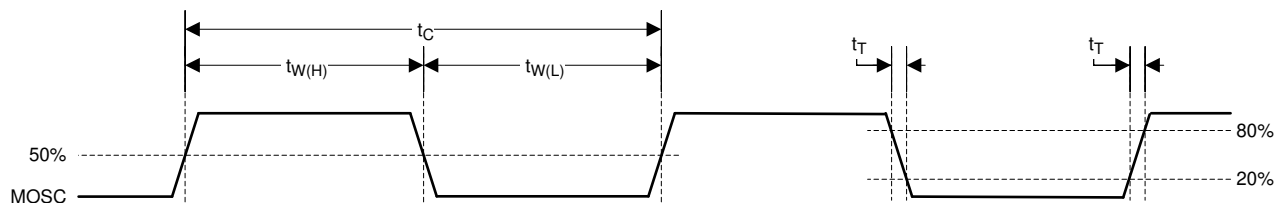
Figure 1. System Oscillators
