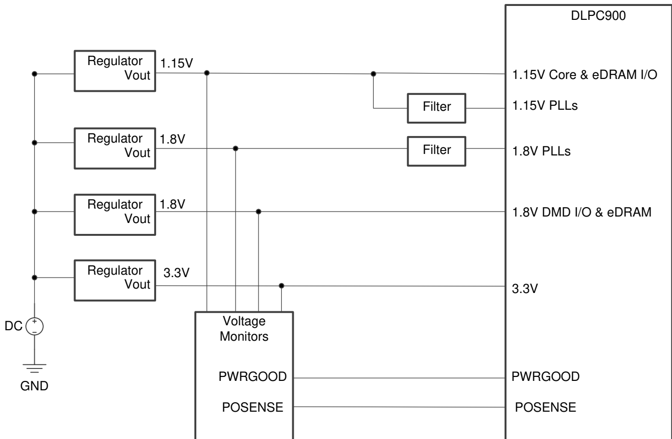
Figure 35. Power Regulation
