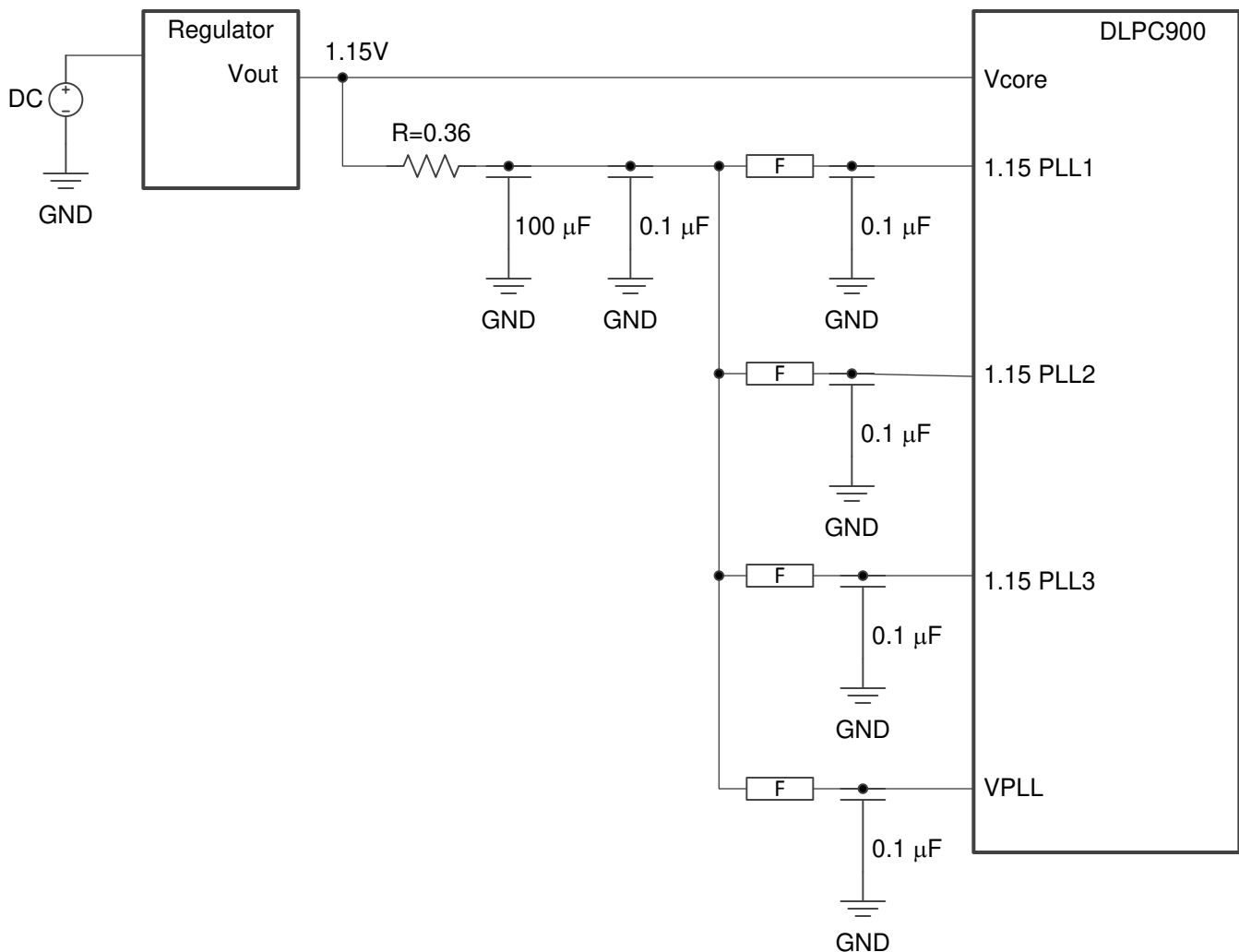
Figure 37. Recommended Filter Topology for PLL 1.15-V Supplies
