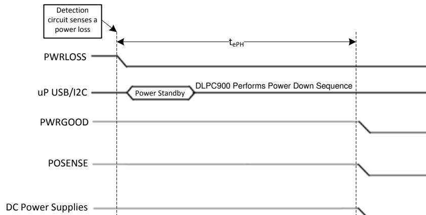
Figure 5. Unanticipated Power Loss Timing Diagram
