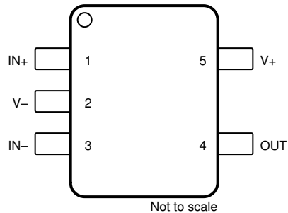
TLV9051 DCK Package 5-Pin SC70 Top View
