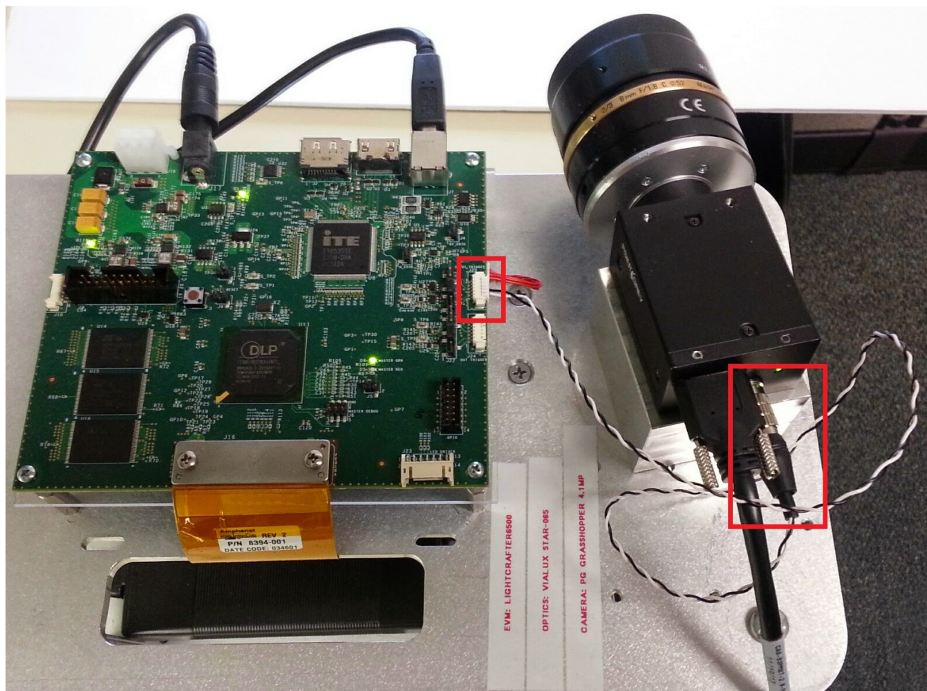
Figure 3-8. Connecting the Camera to the Host PC
