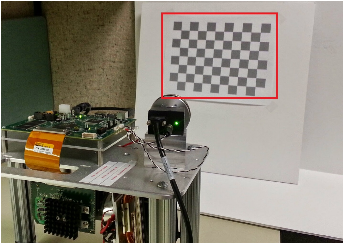
Figure 3-6. Calibration Board Attached to Flat Calibration Surface
