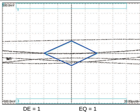
Figure 22. Eye Pattern at A → X = 40"; Y = 2"
