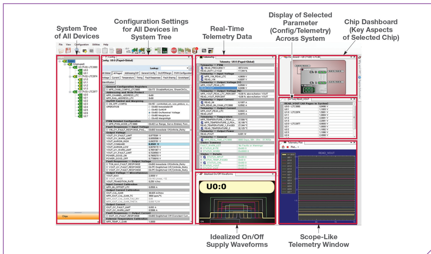
LTpowerPlay GUI
