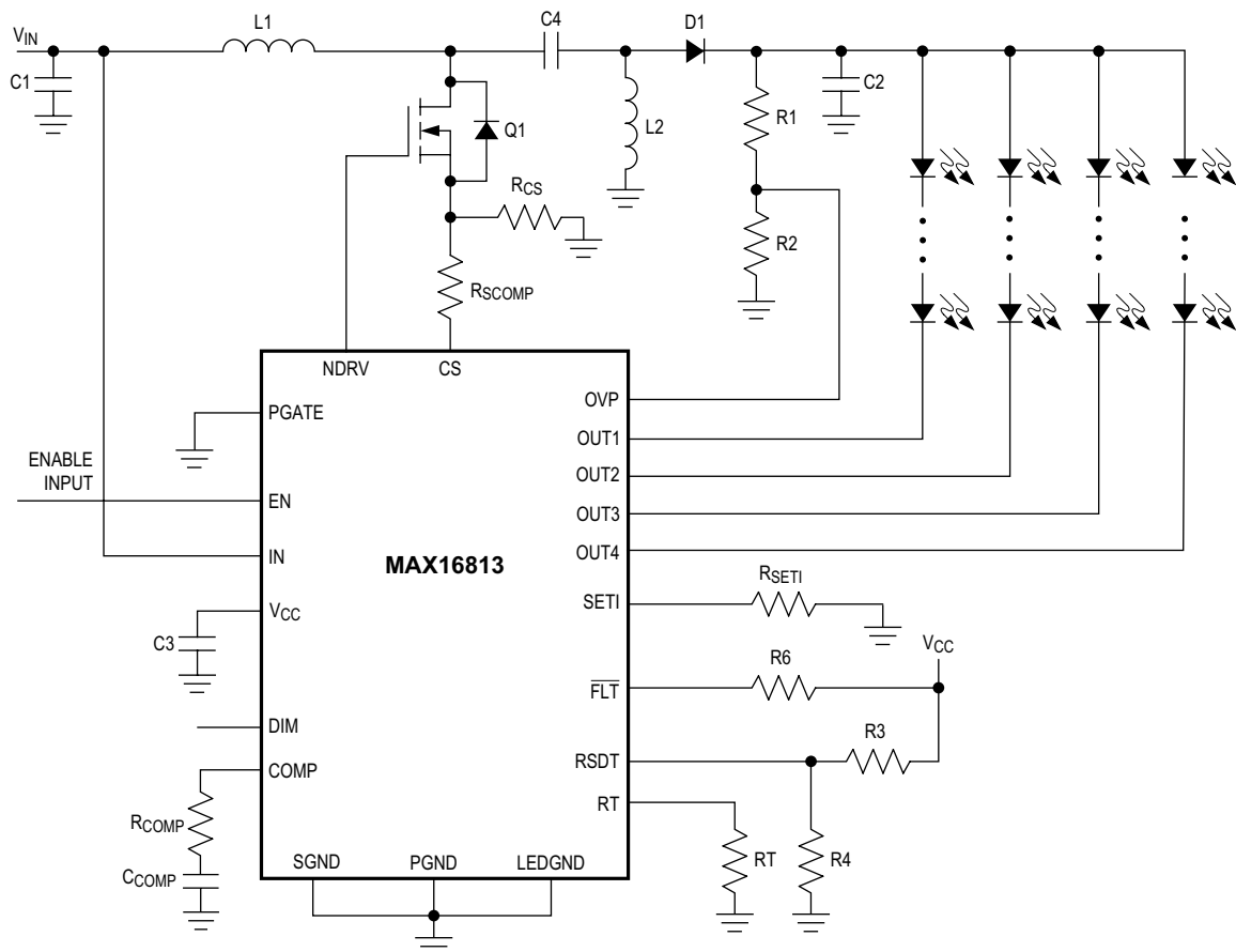
Figure 5. SEPIC LED Driver
