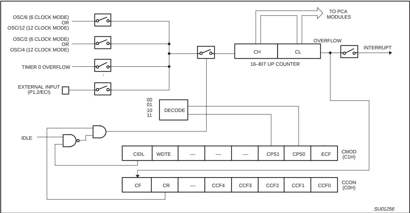
Figure 36. PCA Timer/Counter
