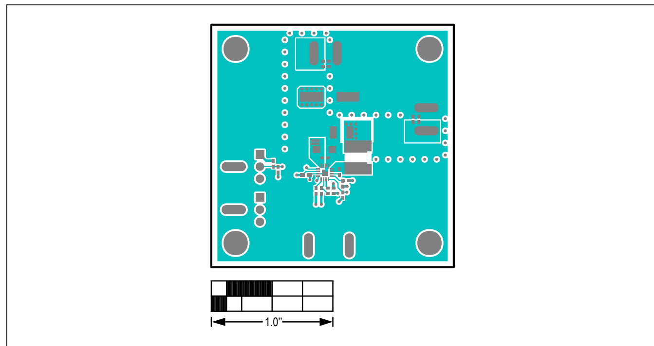
MAX17632B 5V EV Kit—Top Layer
