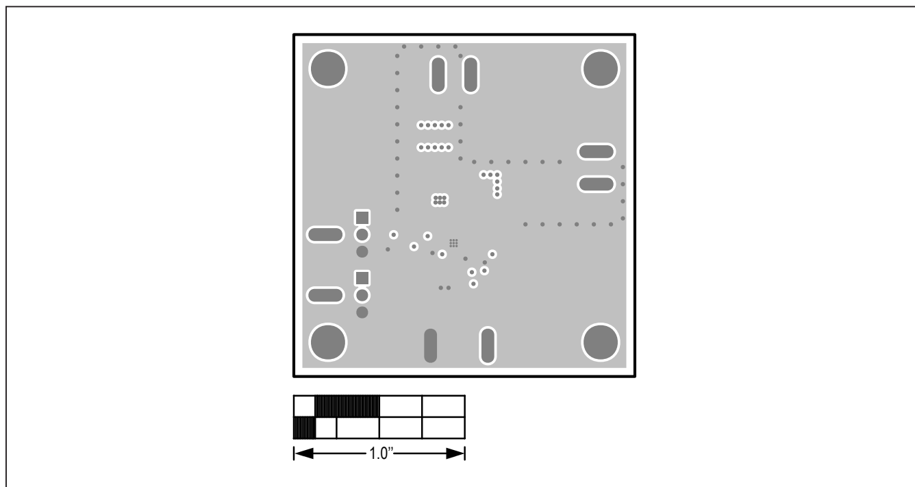
MAX17632B 5V EV Kit—Layer 2
