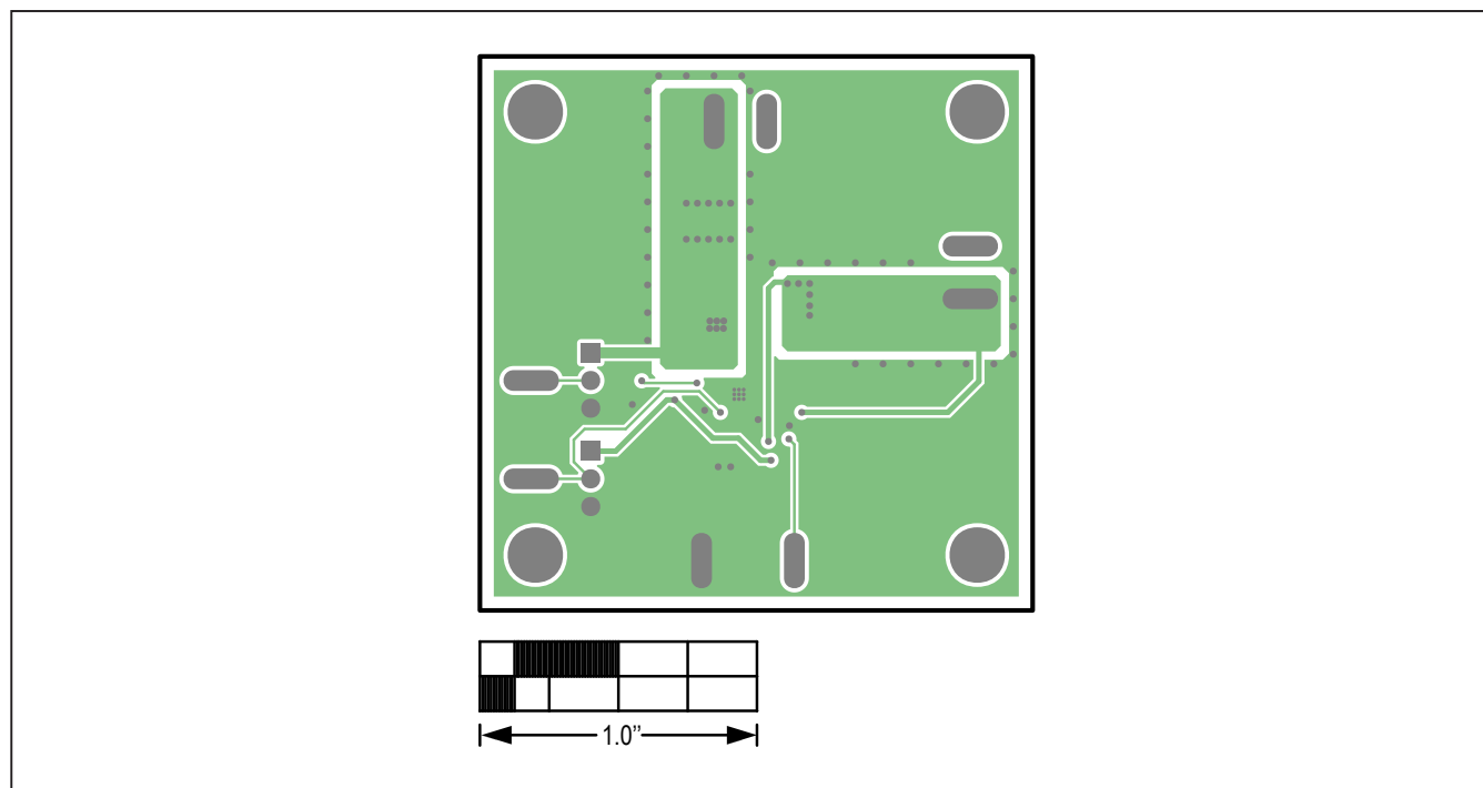
MAX17632B 5V EV Kit—Layer 3
