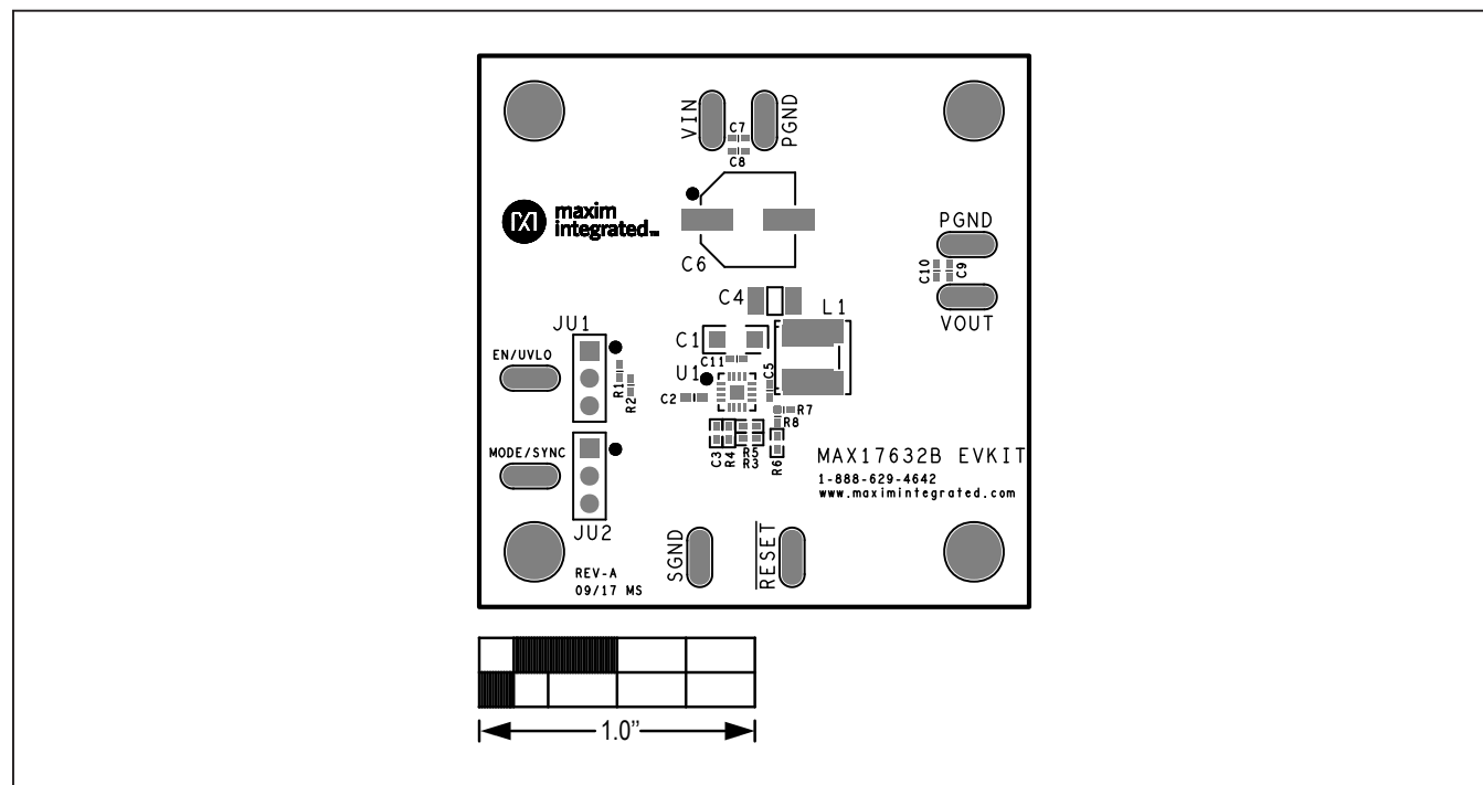
MAX17632B 5V EV Kit—Top Silkscreen
