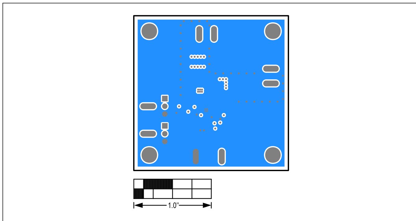
MAX17632B 5V EV Kit—Bottom Layer
