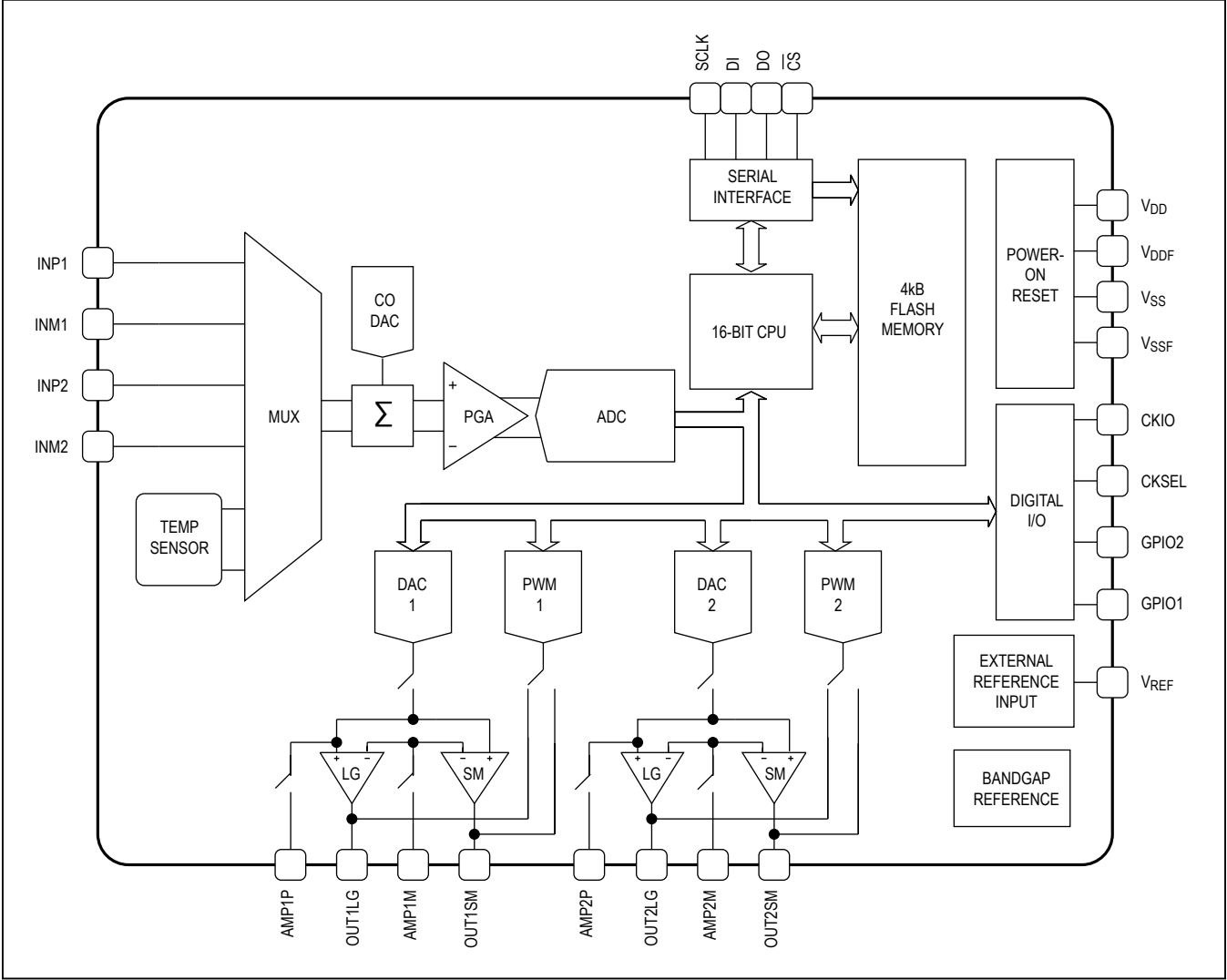
Functional Diagram
