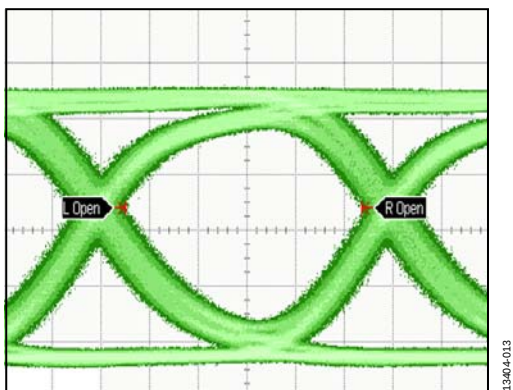
Figure 13. 1000 Waveforms and Persist Mode at 11.3 Gbps
