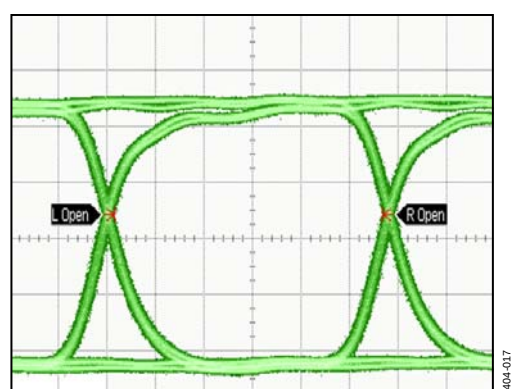
Figure 17. 1000 Waveforms and Persist Mode at 4.25 Gbps
