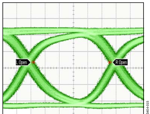
Figure 15. 1000 Waveforms and Persist Mode at 9.953 Gbps
