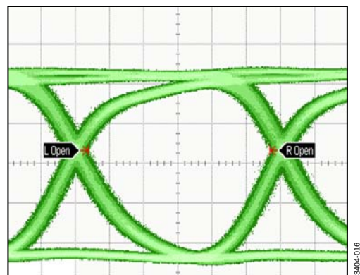
Figure 16. 1000 Waveforms and Persist Mode at 8.5 Gbps
