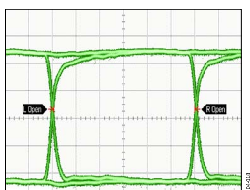
Figure 18. 1000 Waveforms and Persist Mode at 1.25 Gbps
