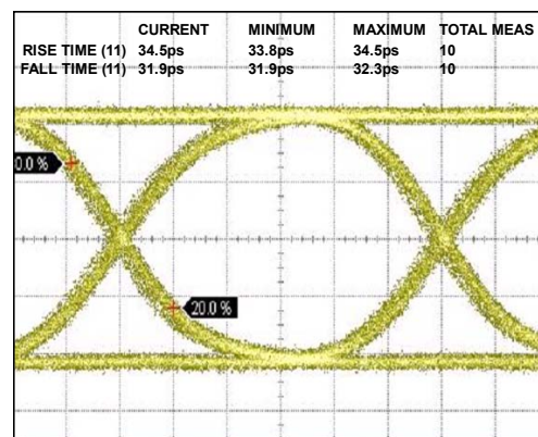
Figure 5. A Reference Eye at 9.953 Gbps
