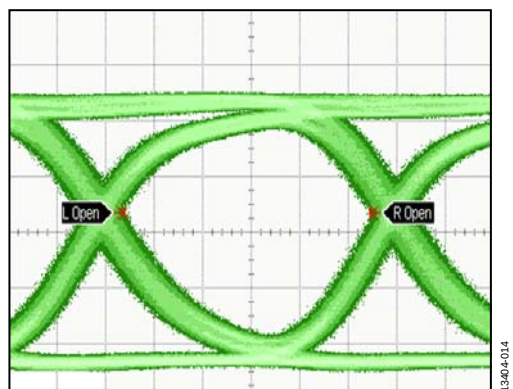
Figure 14. 1000 Waveforms and Persist Mode at 10.3 Gbps
