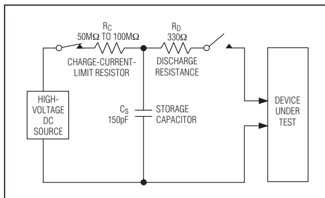
Figure 1c. IEC 61000-4-2 ESD Test Model
