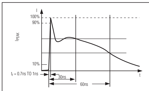
Figure 1d. IEC 61000-4-2 ESD Generator Current Waveform
