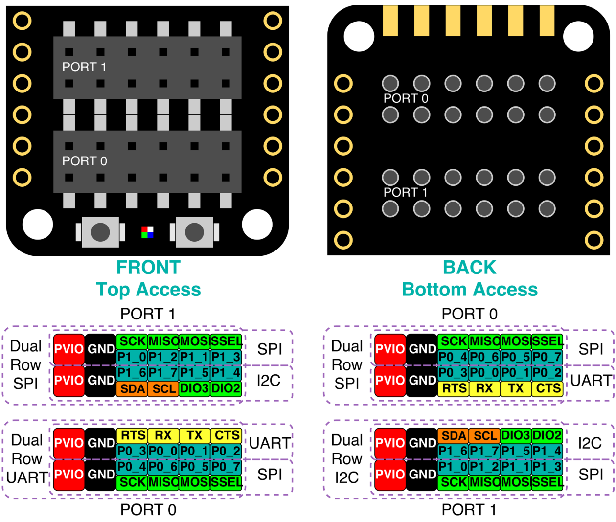
Figure 3. Pmod Port Pinouts
