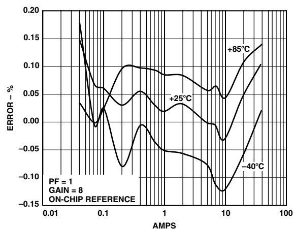
TPC 3. Error as a % of Reading (Gain = 8)
