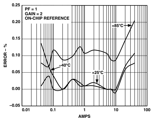
TPC 2. Error as a % of Reading (Gain = 2)
