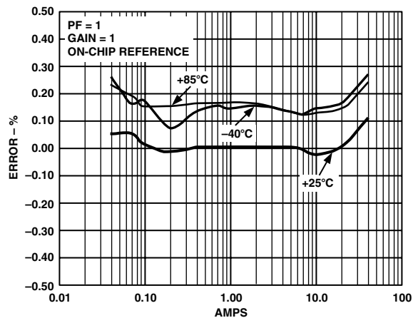
TPC 1. Error as a % of Reading (Gain = 1)
