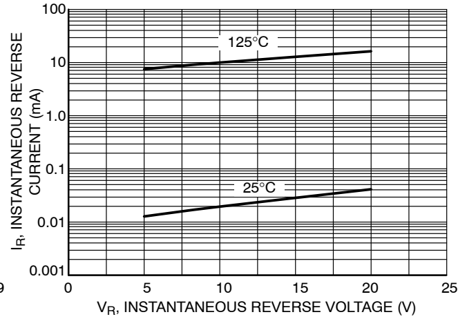
Figure 9. Schottky Typical Reverse Current vs. Reverse Voltage
