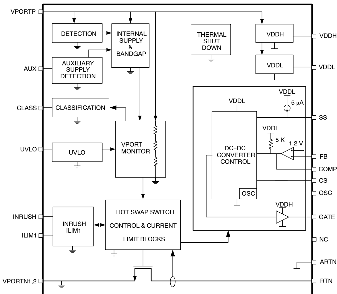
Figure 1. NCP1082 Block Diagram
