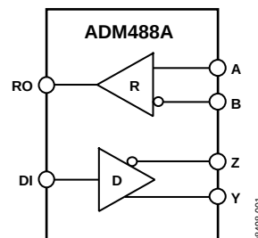
Figure 1. ADM488A
