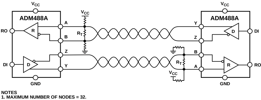
Figure 20. ADM488A/ADM489A Full-Duplex Data Link
