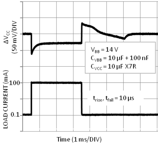
Figure 8. Load Transient Response ( I_{CC} 100 \mu\text{A} to 100 mA)
