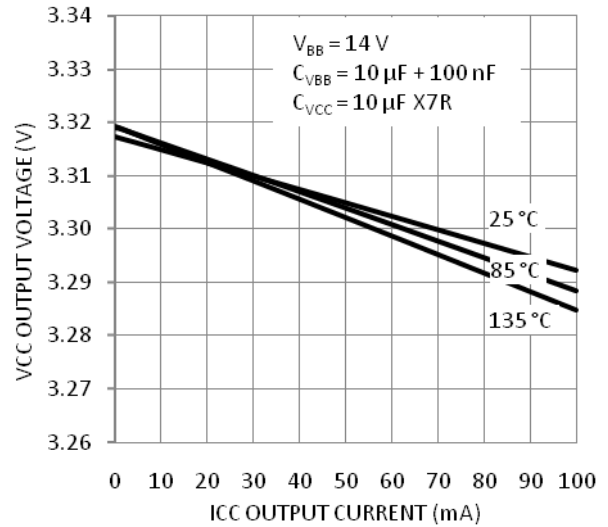
Figure 13. Output Voltage vs. Output Current
