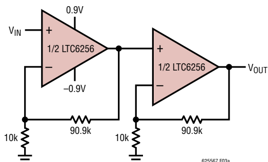
200kHz 130 \mu A Gain-of-100 Amplifier
