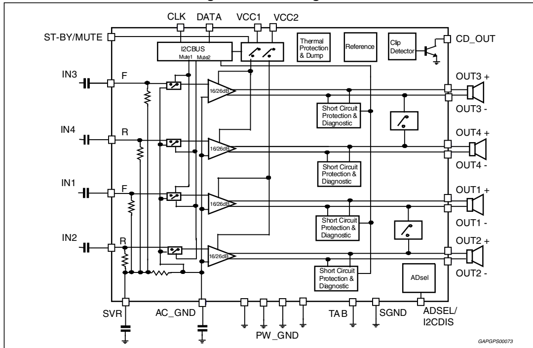
Figure 2. Block diagram
