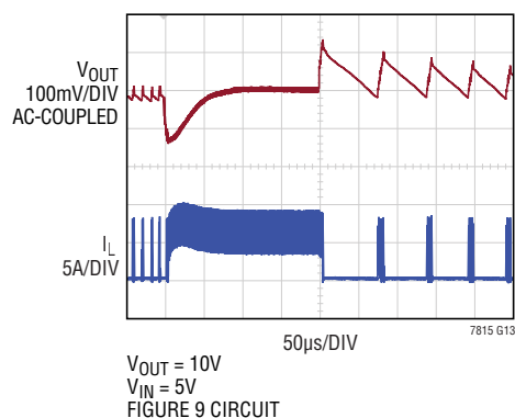
Load Step (Boost) Burst Mode Operation
