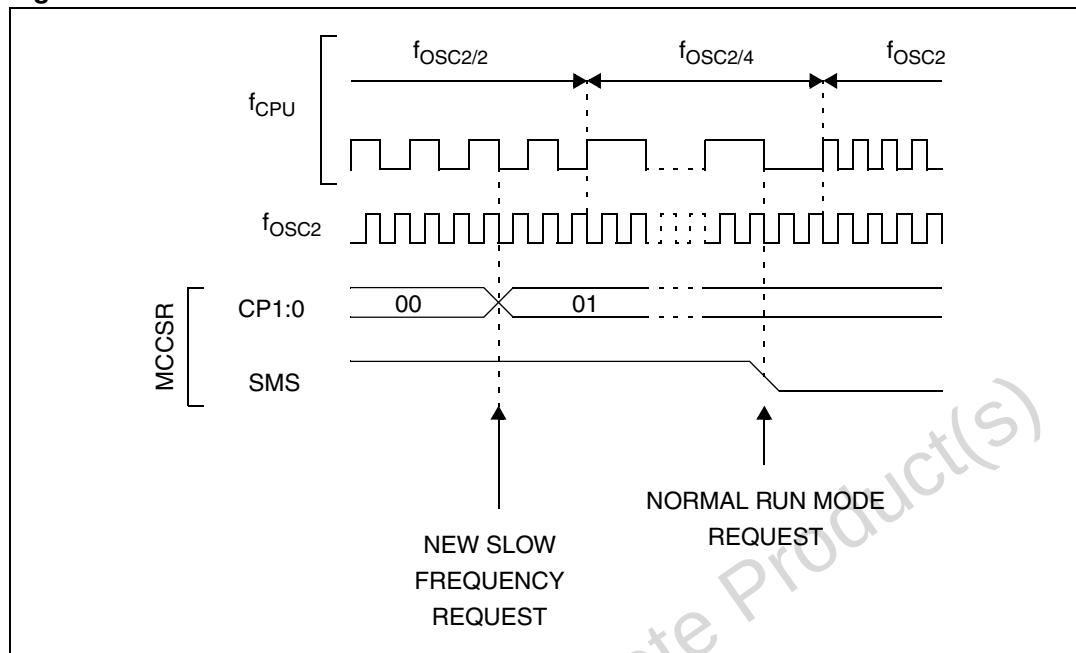
Figure 23. Slow mode clock transitions
