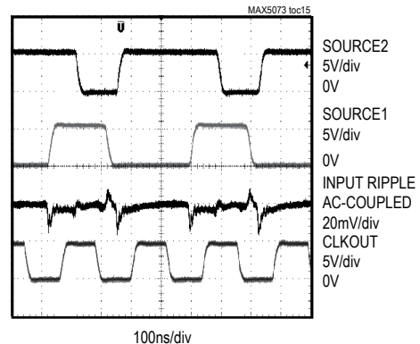
OUT-OF-PHASE OPERATION
