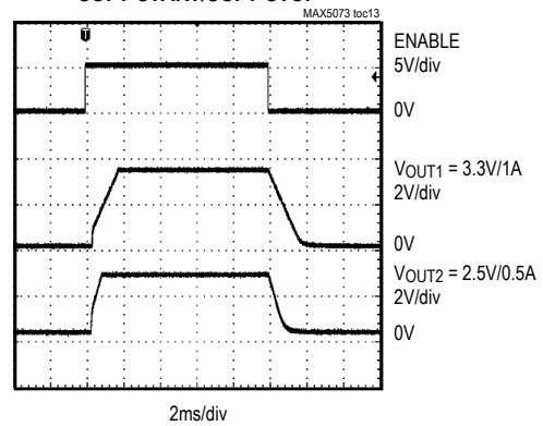
SOFT-START/SOFT-STOP
