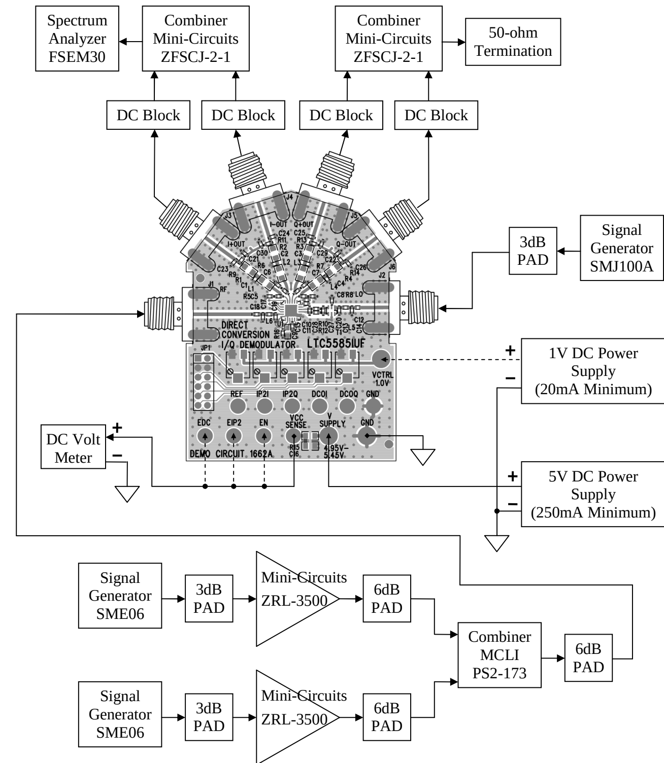
Figure 1. Measurement Setup
