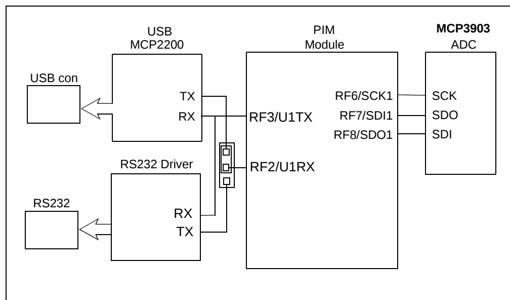
FIGURE 1-5: Serial Communication Block Diagram.
