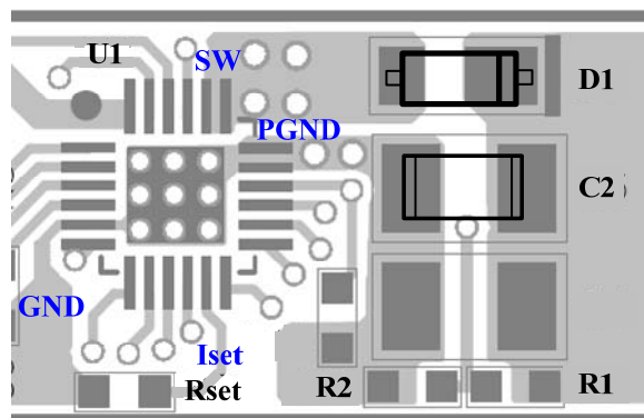
Figure 10: Sample Layout
