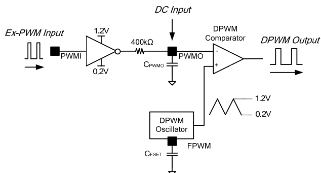
Figure 5: PWM Dimming
