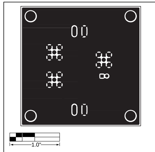
Figure 4. MAX4444 EV Kit PC Board Layout—Solder Side
