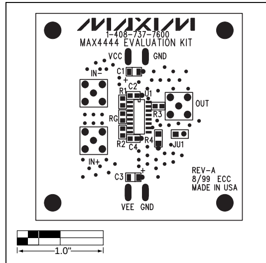
Figure 2. MAX4444 EV Kit Component Placement Guide—Component Side
