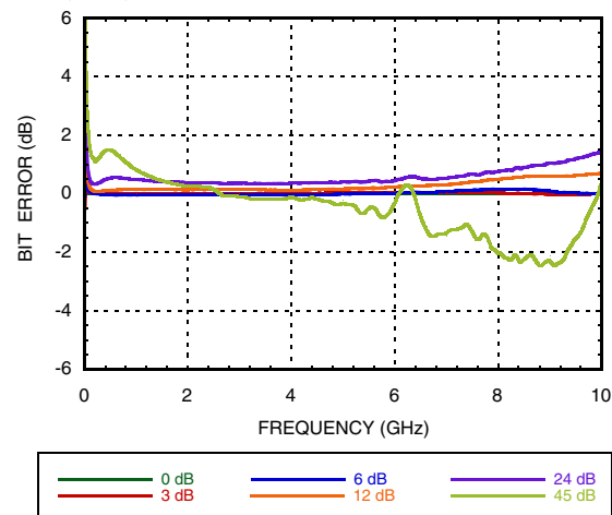
Bit Error vs. Frequency
