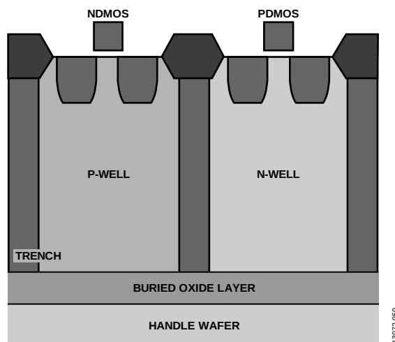
Figure 53. Trench Isolation
