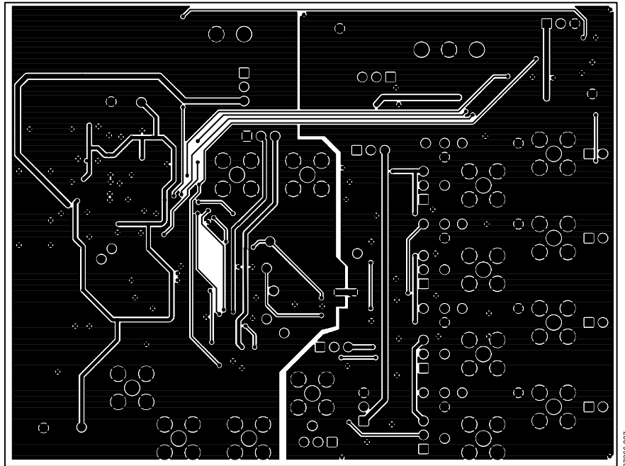
Figure 7. Solder Side PCB Drawing
