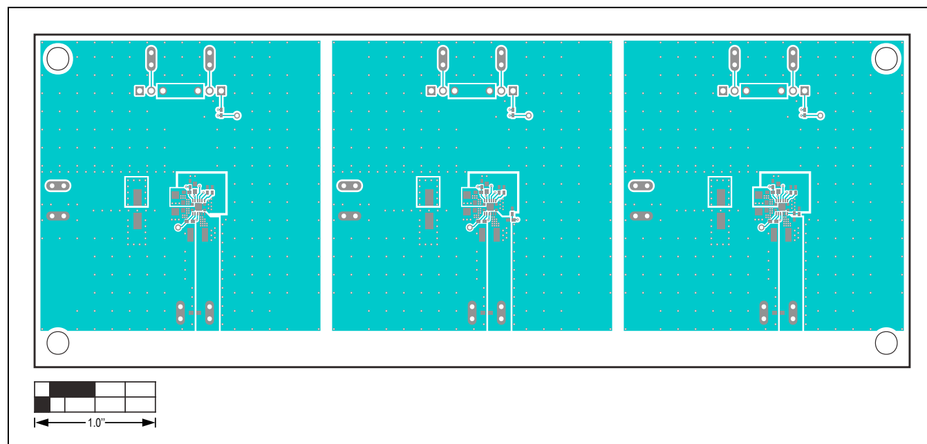
MAXM17630/MAXM17631/MAXM17632 EV Kits—Top Layer
