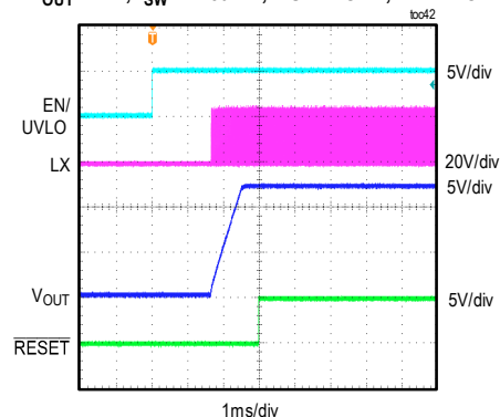
MAXM17631 STARTUP THROUGH ENABLE V_{OUT} = 12V , f_{SW} = 2150kHz , FULL LOAD, PWM MODE
