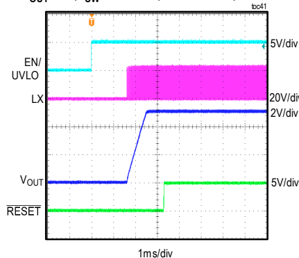
MAXM17631 STARTUP THROUGH ENABLE V_{OUT} = 5V , f_{SW} = 1250kHz , FULL LOAD, PWM MODE
