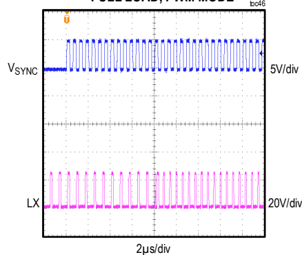
MAXM17631 EXT CLOCK SYNC V_{OUT} = 5V , f_{SW} = 1.25MHz , f_{SYNC} = 1.75MHz , FULL LOAD, PWM MODE
