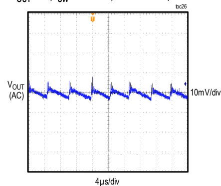
MAXM17631 STEADY-STATE OUTPUT-VOLTAGE RIPPLE V_{OUT} = 5V , f_{SW} = 1250kHz , 10mA LOAD, DCM MODE
