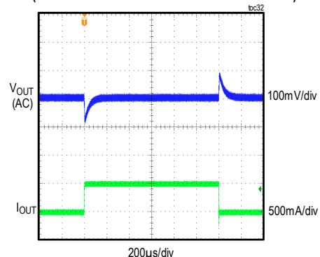
MAXM17631 LOAD TRANSIENT RESPONSE V_{OUT} = 5V , f_{SW} = 1250kHz , PWM MODE (LOAD CURRENT STEPPED FROM 0A TO 0.5A)
