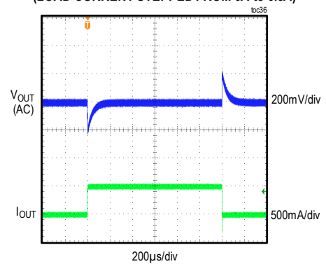
MAXM17632 LOAD TRANSIENT RESPONSE V_{OUT} = 12V , f_{SW} = 2150kHz , PFM MODE (LOAD CURRENT STEPPED FROM 10mA TO 0.5A)
