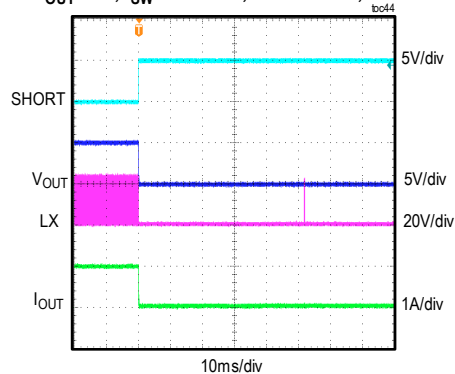
MAXM17631 OUTPUT SHORT IN STEADY-STATE V_{OUT} = 5V , f_{SW} = 1250kHz , FULL LOAD, PWM MODE
