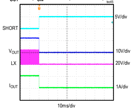
MAXM17632 OUTPUT SHORT IN STEADY-STATE V_{OUT} = 12V , f_{SW} = 2150kHz , FULL LOAD, PWM MODE
