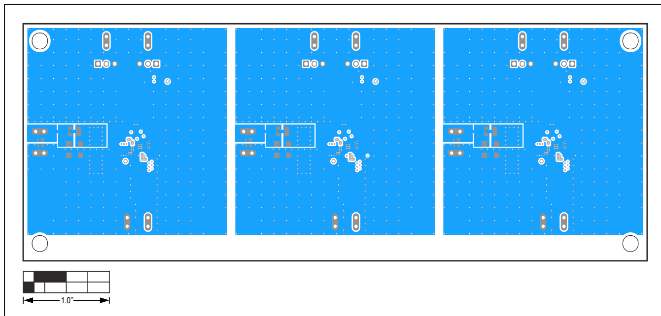
MAXM17630/MAXM17631/MAXM17632 EV Kits—Bottom Layer
