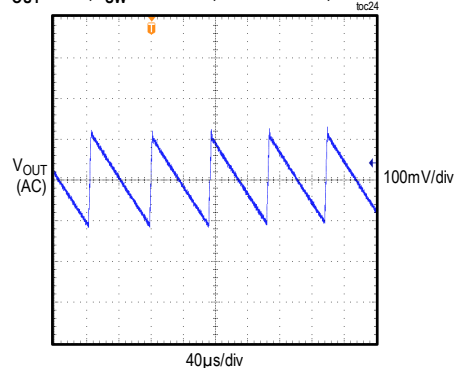
MAXM17632 STEADY-STATE OUTPUT-VOLTAGE RIPPLE V_{OUT} = 12V , f_{SW} = 2150kHz , 10mA LOAD, PFM MODE
