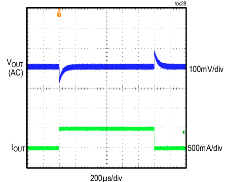
MAXM17630 LOAD TRANSIENT RESPONSE V_{OUT} = 3.3V , f_{SW} = 900kHz , PWM MODE (LOAD CURRENT STEPPED FROM 0A TO 0.5A)
