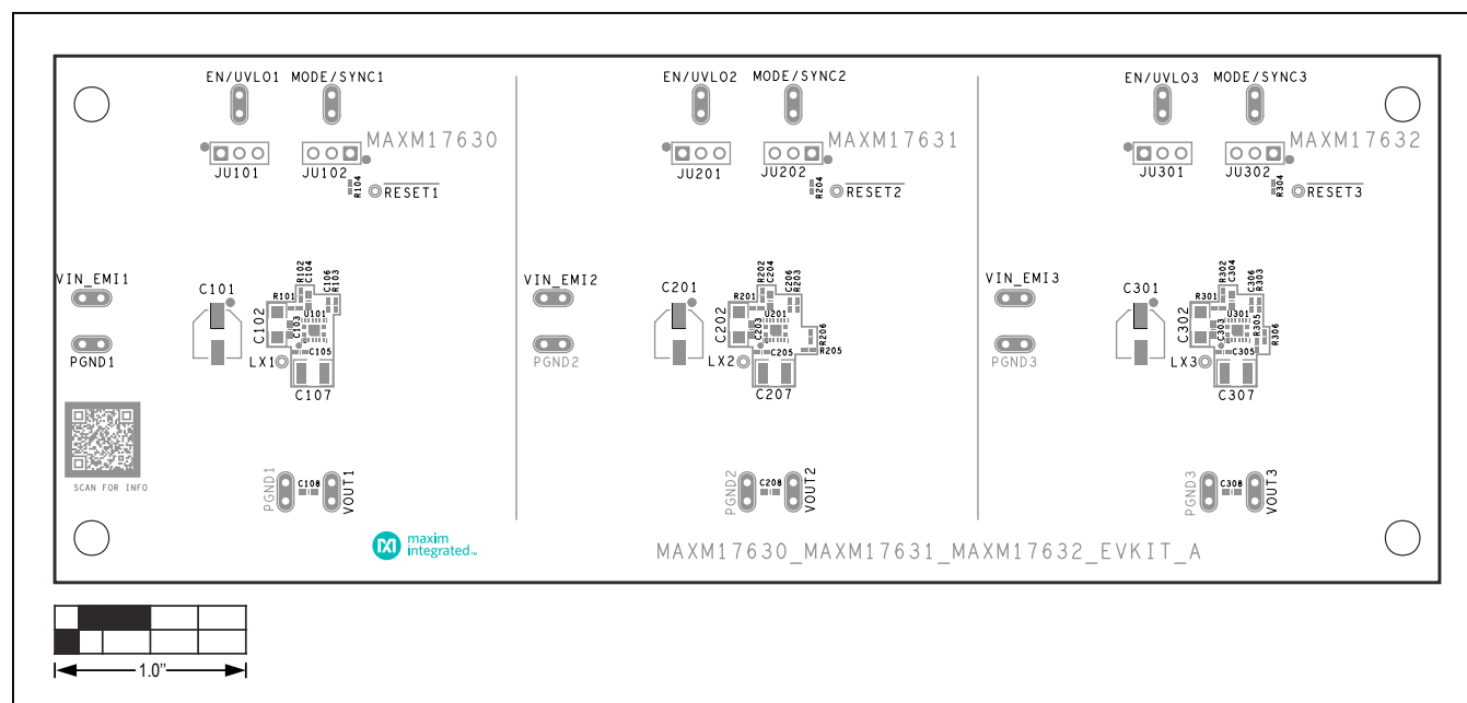
MAXM17630/MAXM17631/MAXM17632 EV Kits—Top Silkscreen
