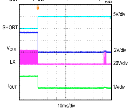
MAXM17630 OUTPUT SHORT IN STEADY-STATE V_{OUT} = 3.3V , f_{SW} = 900kHz , FULL LOAD, PWM MODE
