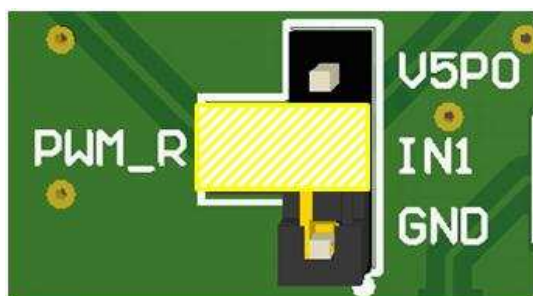
Figure 5. IN1 Connected to PWM Output
